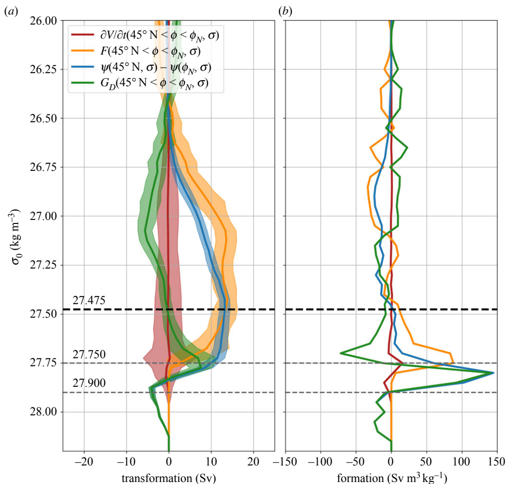
Figure 2. (a) Time-mean diapycnal water mass transformation and overturning for the region between 45^\circ \text{ N} and the Greenland–Scotland Ridge/Davis Strait ( \phi_N ) from Estimating the Circulation and Climate of the Ocean version 4 (ECCO v4) [10]. The plot shows the surface water mass transformation, F(45^\circ \text{ N} < \phi < \phi_N, \sigma) (orange line); the overturning, \Psi(45^\circ \text{ N}, \sigma) - \Psi(\phi_N, \sigma) (blue line); and the volume change below isopycnal \sigma , \partial V/\partial t(45^\circ \text{ N} < \phi < \phi_N, \sigma) (red line). The green line indicates the residual, which is interpreted as the diapycnal water mass transformation due to mixing, G_D(45^\circ \text{ N} < \phi < \phi_N, \sigma) . The shading represents the standard deviation of the annual means. The dashed black line is at the density of the maximum overturning, \sigma_{\text{MOC}} . The overturning is shown separately for 45^\circ \text{ N} and the Greenland–Scotland Ridge in electronic supplementary material, figure S1. (b) The convergence in density space of the terms in (a), with positive values indicating that a given term creates waters within a density class.
