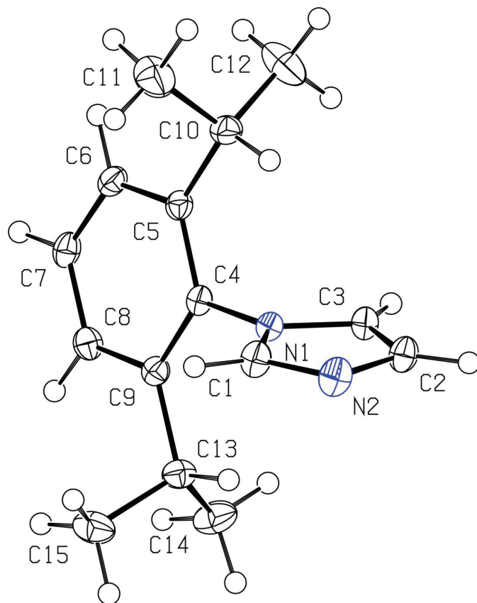
Figure 1 View of one molecule of Dipp Im with 50% probability ellipsoids.
