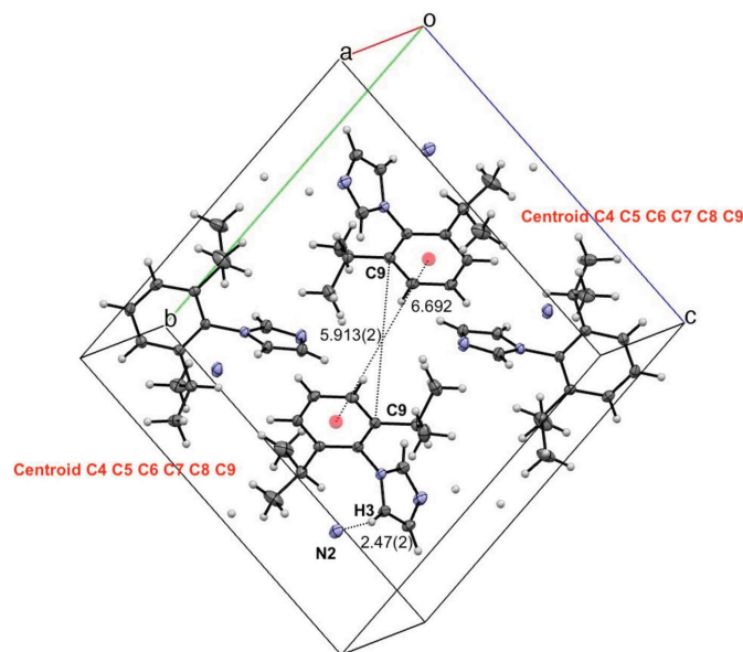
Figure 2 View of four molecules of Dipp Im in the unit cell with 50% probability ellipsoids, highlighting intermolecular distances and close contacts. Distances between centroids (red circles) are listed without standard deviations because these positions were calculated.
