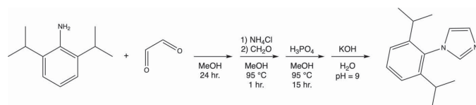
Figure 3 Reaction scheme.
