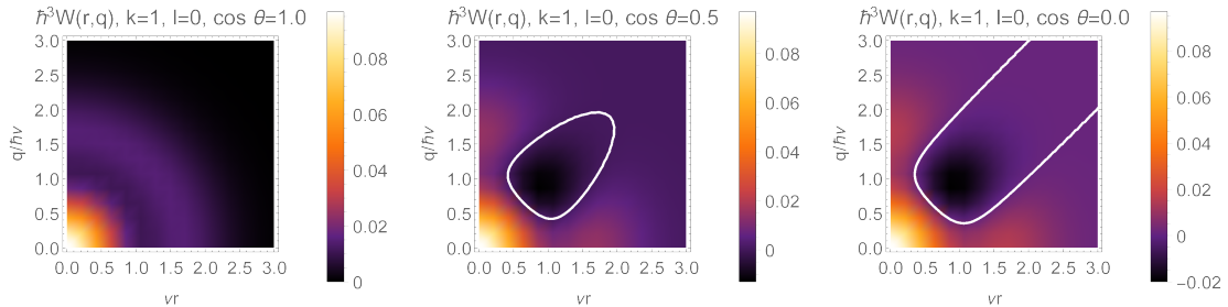
Figure 1: Phase-space distributions W_{10} for quantum numbers k = 1, l = 0 as functions of r = |\mathbf{r}| and q = |\mathbf{q}| . The white lines indicate nodes where W_{10} = 0 . Distributions are shown for several values of the angle \theta given by \cos \theta = \mathbf{r} \cdot \mathbf{q} / r q .
