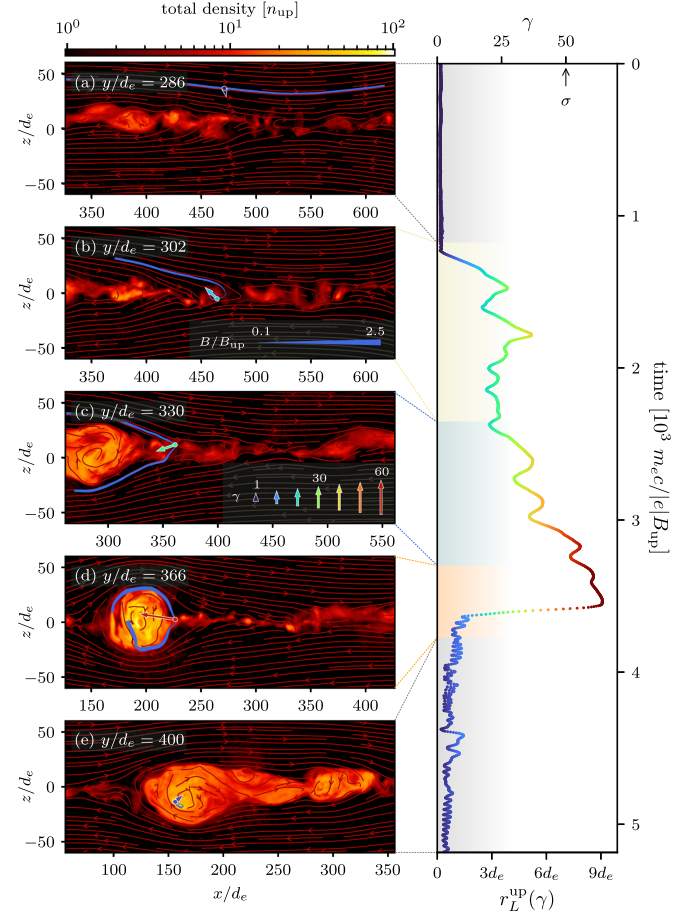
Figure 9. Time evolution of a typical accelerated electron in the strongly cooled simulation. The right-hand panel shows the energy evolution of the particle with time. Panels (a)–(e) show the density slice and the magnetic field lines in the x - z plane at a particular time of the simulation (corresponding to the right-hand panel). The position and the velocity of the electron are shown with a colored circle and an arrow (color corresponds to its energy at that particular time). The magnetic field line passing through the position of the particle is shown as a blue line, with its thickness corresponding to the strength of the magnetic field. The electron starts cold upstream of the current layer (a) and is accelerated to the Lorentz factor up to \approx \sigma in the current sheet (b), after which it is picked up by the outflow from the X-point and gains further energy (c). Ultimately, the electron experiences an intensive slow-down when it collides with the magnetic field inside the plasmoid (d), where it remains throughout the rest of its lifetime (e).
