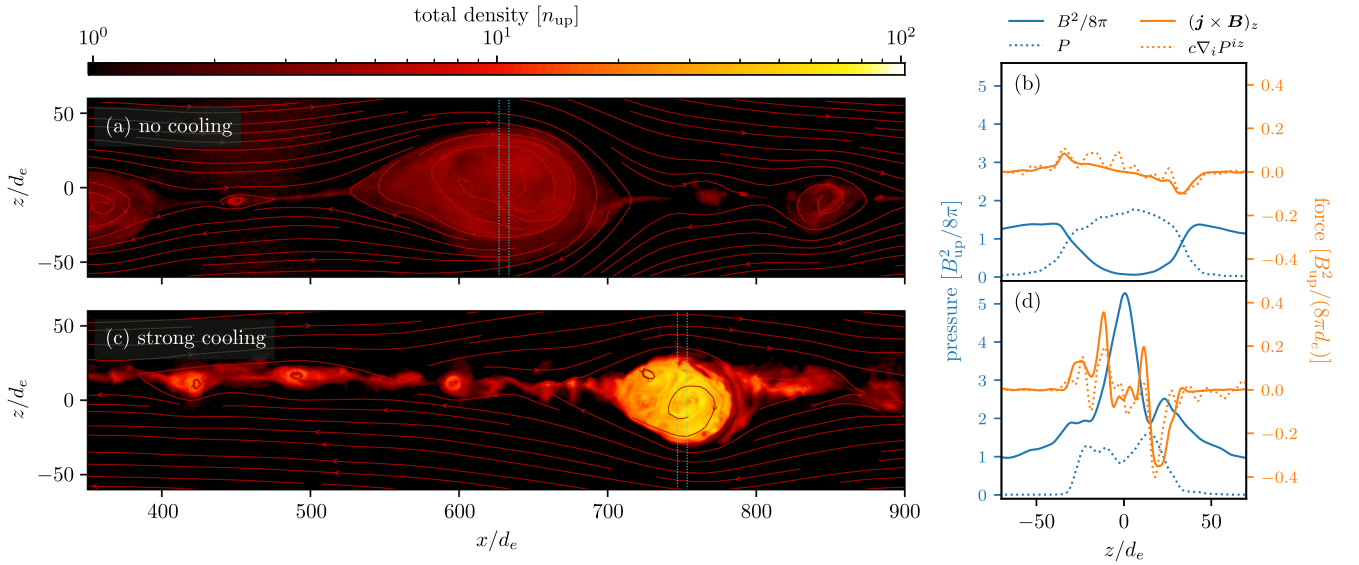
Figure 4. A cross-section of typical plasmoids for uncooled ((a), (b)) and strongly cooled ((c), (d)) current sheets. The left-hand column ((a), (c)) shows density slices and the magnetic field lines. The region highlighted with a cyan-dotted boundary is shown in 1D cuts in ((b), (d)), where we plot the magnetic field, B^2/8\pi , and gas pressure, P , with the corresponding magnetic tension force, (\mathbf{j} \times \mathbf{B})_z , and the gradient of the pressure tensor, c\nabla_z P^{iz} . On the one hand, in the uncooled case, the plasmoids are in equilibrium in terms of magnetic and thermal pressure, with the thermal pressure typically dominating inside the plasmoids. On the other hand, the equilibrium inside the cooled plasmoids is more dynamic, with the magnetic field pressure being larger than the upstream value, and dominating the plasmoid cores.
