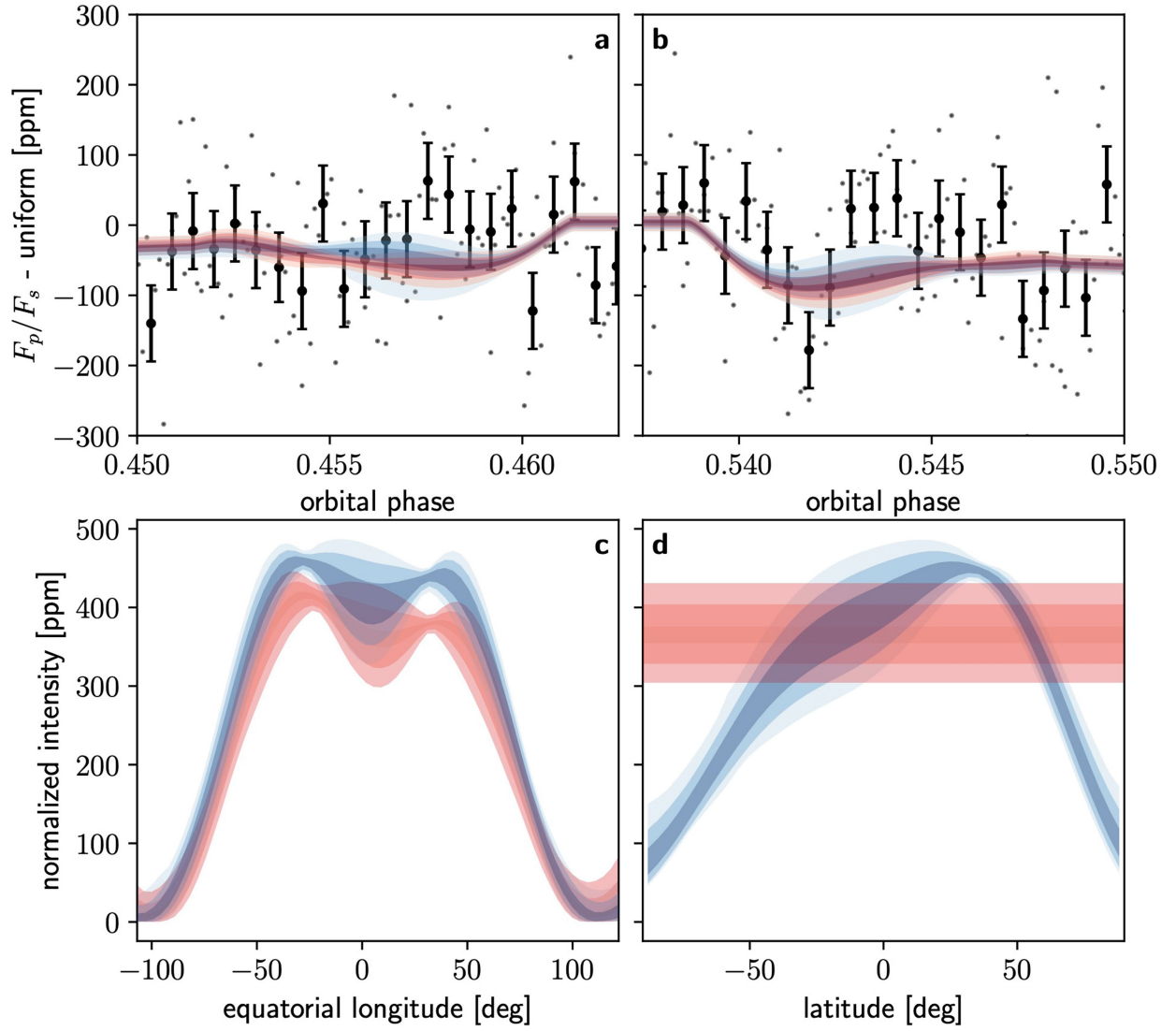
Extended Data Fig. 9 | Latitudinal structure in the eclipse map. a , Ingress of the eclipse, with two models overplotted and a 1,096 ppm (white-light planet flux at mid-eclipse) uniform planet model subtracted to highlight deviations. The data (small dots) have been binned by a factor of five (dots with 1\sigma error bars) for clarity. The blue model is the eclipse map for l_{\max} = 5, N = 5 presented in the text. The red model uses a constant-with-latitude Fourier series as the basis set, rather than spherical harmonics, to investigate constraints on latitudinal
