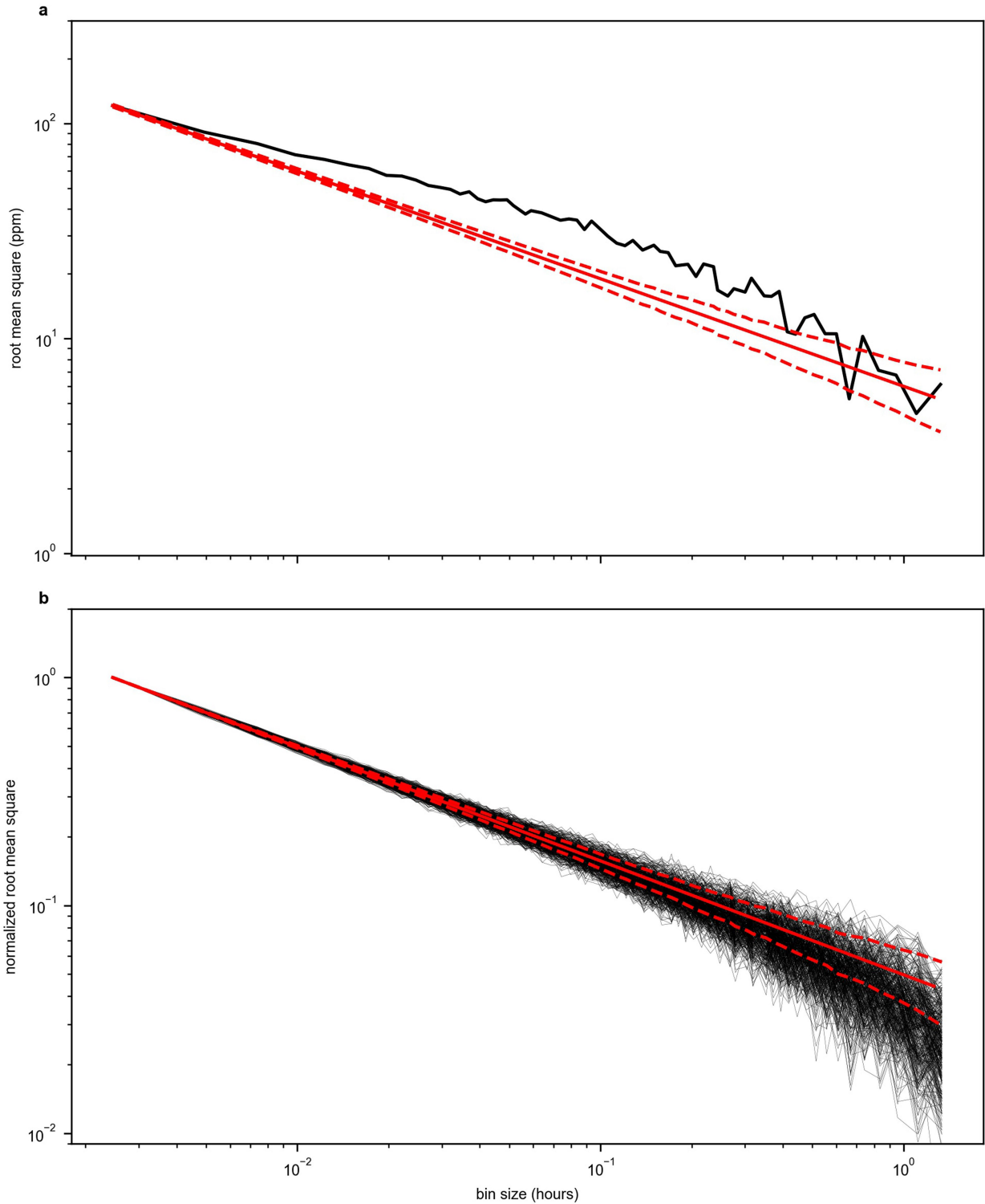
Extended Data Fig. 4 | Light-curve residuals binned in time. a , Absolute root mean square (RMS) of the residuals as a function of bin size (black line) for the white-light curve. The RMS values are plotted against the Poisson noise limit (red line), which decreases as the square root of the number of integrations contained in a single bin. We also show the theoretical 1\sigma error envelope of the Poisson noise. The residuals bin down to about 5 ppm for bins of 1 h and show no evidence of a noise floor, similar to what was observed from commissioning data 54 . The broadband residuals do not perfectly follow the Poisson noise,
