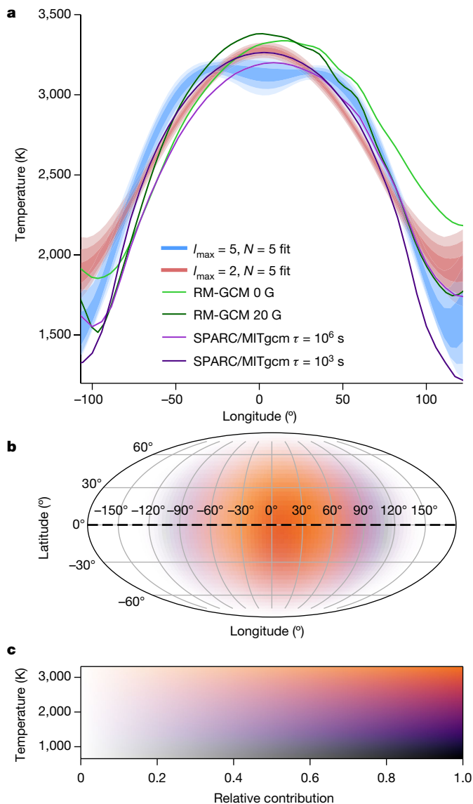
Fig. 4 | Retrieved temperature map of WASP-18b. a , Latitudinally averaged brightness temperatures (see Methods) of the planet along the equator. The blue and red shaded areas show solutions for I_{\max} = 5, N = 5 and I_{\max} = 2, N = 5 (see Methods), respectively. The effective broadband wavelength of the map, weighted by the observed flux ( F_p + F_s ) and instrument response, is \lambda = 1.27 \mu\text{m} . Statistically, the blue model is marginally preferred. Dark, medium and light shading denote the 1\sigma , 2\sigma and 3\sigma confidence regions, respectively, showing the range of model possibilities. Overplotted are several predictions from GCMs with magnetic field 52 (green) or uniform 53 (purple) drag timescales (see Methods). The plot only shows longitudes emitting at least 10% of the substellar flux. b , The temperature map of WASP-18b for the I_{\max} = 5, N = 5 solution. Along the equator at -90^\circ , 0^\circ and 90^\circ longitude, the temperatures are 1,744 K, 3,121 K and 2,009 K, respectively. c , The colour bar for the map shown in b . Colour represents the brightness temperature and saturation represents the relative contribution to the light curve based on its visibility.
