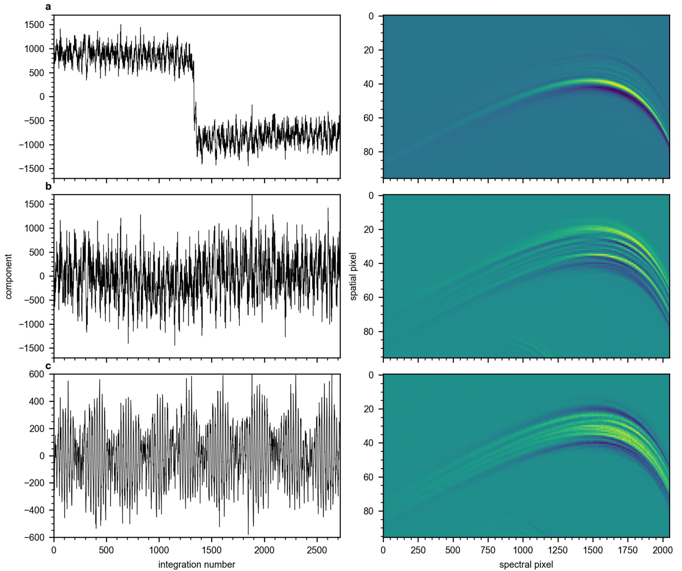
Extended Data Fig. 2 | Morphological changes of the spectral trace on the NIRISS detector as identified through PCA on the time series of the detector images. a, First principal component with its eigenvalues (left) and its corresponding eigenimage (right). The tilt event occurring near the 1,336th integration can clearly be identified as the largest source of variance to the detector images. It results in a subtle change to the trace profile in the cross-dispersion direction, predominantly visible near its lower edge of the trace. b, Second principal component with its eigenvalues (left) and its corresponding
