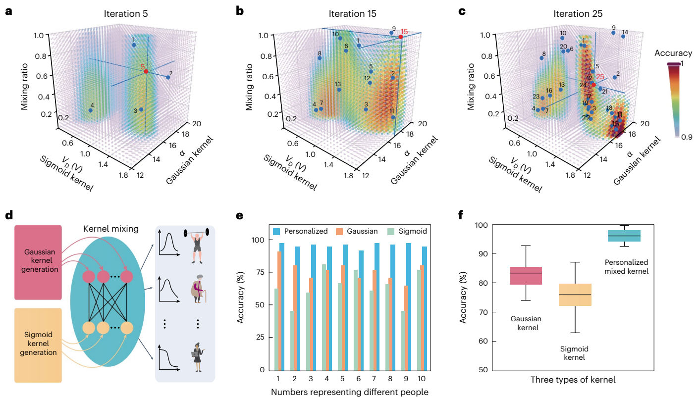
Fig. 3 | BO of personalized mixed kernels. a–c, BO of the Gaussian kernel hyperparameter, sigmoid kernel hyperparameter and mixing ratio after 5 (a), 15 (b) and 25 (c) iterations. d, Schematic of personalized SVM classification enabled by using two MKH transistors to generate a complete set of mixed kernels. e, Arrhythmia detection accuracy comparison for SVMs using only a Gaussian kernel, only a sigmoid kernel or a personalized mixed kernel for ten different
