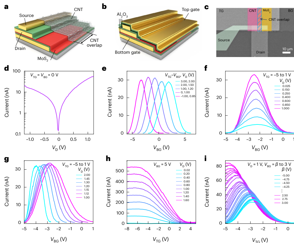
Fig. 1 | MKH transistor schematic, structure and performance. a , Partial schematic of the device showing the MoS 2 /CNT channels and overlap. b , Full schematic of a completed device. c , Electron microscopy image of the fabricated device with the device regions labelled. d , I_D – V_D curve of the device with both top and bottom gates grounded. e , I_D – V_{BG} curves of the device in the Gaussian operation mode showing tunable \mu . f , I_D – V_{BG} curves of the device in the Gaussian
