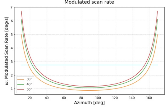
FIG. 1. Plot of the modulated azimuthal scan rate in ^{\circ}/s with respect to the azimuth coordinate of the telescope at 30, 40, 50° elevations. A base scan rate of 0.75^{\circ}/s is used. The blue line indicates the desired maximum scan rate of 2.75^{\circ}/s .
