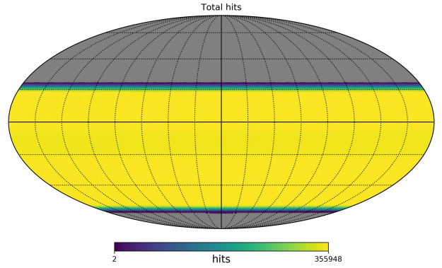
FIG. 2. A hitmap of a yearlong Modulated High Cadence Survey Strategy schedule observing at 40° elevation, [21^{\circ}, 159^{\circ}] azimuth range and no Sun-Moon avoidance. Note the uniformity in observation depth.
