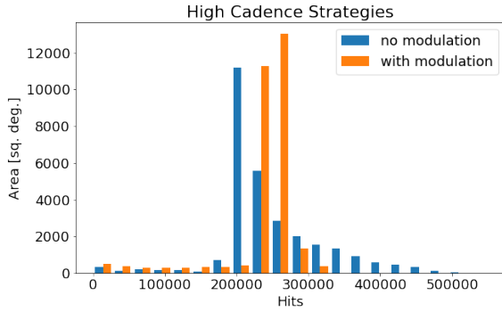
FIG. 5. A histogram of hits for the High Cadence Survey Strategy maps in Figure 4, with the map without velocity modulation in blue and the Modulated High Cadence strategy map in orange.
