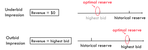
Fig. 1: Optimal Reserve Prices for Two Cases
