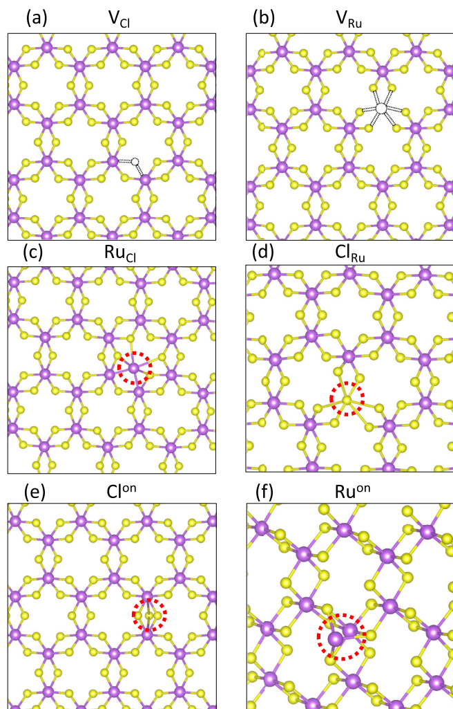
FIG. 2. Top view of the atomic structure of point defect. (a) Single Cl atom vacancy ( V_{\text{Cl}} ), (b) single Ru atom vacancy ( V_{\text{Ru}} ), (c) a Ru atom takes the place of a Cl atom ( \text{Ru}_{\text{Cl}} ), (d) a Cl atom takes the place of a Ru atom ( \text{Cl}_{\text{Ru}} ), (e) an excess Cl atom locates on the top of the layer ( \text{Cl}^{\text{on}} ), (f) an excess Ru atom locates on the top of the layer ( \text{Ru}^{\text{on}} ). The missing atom is marked by black dashed lines in (a) and (b). The red dashed circle is used to guide readers' eyes to the point defect.
