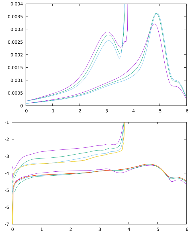
FIG. 28. As in Fig. 26, but now for \bar{C} .
