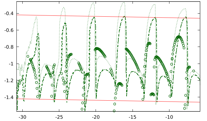
FIG. 11. The mass scaling function f_M for \epsilon_2 = 0.75 , at the same four resolutions as in Fig. 10. The red straight lines have slope \delta\gamma = -0.0016 , taken from the fit in Fig. 10. f_M is both not periodic enough and too resolution-dependent for a meaningful fit to its average slope, but \delta\gamma = -0.0016 is consistent with the data.
