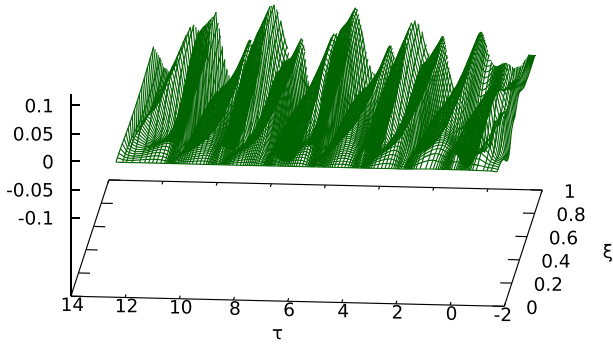
FIG. 16. Surface plot of the scaled nonspherical scalar field component \epsilon_2^{-1}e^{-\kappa\tau}\psi_2(x, \tau) , in the sub15 evolution of the \epsilon_2 = 0.75 family. Otherwise as described in Fig. 3. Note that the dark green curves in Fig. 14 are the projection of this surface plot in the \xi direction.
