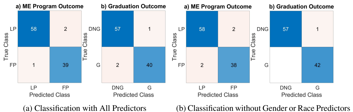
Figure 1: Classification Results
