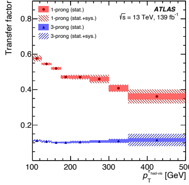
Figure 1: Transfer factors used in the jet-background estimation as a function of p_T^{\tau_{\text{had-vis}}} , for 1-prong (circles) and 3-prong (upward triangles) \tau -lepton decays. The uncertainty due to the limited number of events in CR2 and CR3 is shown as solid filled areas while the hatched areas indicates the total statistical and systematic uncertainties.
