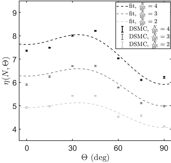
FIG. 9. Plot of \eta vs \Theta from a cross-dimensional rethermalization experiment. The data points (points with error bars) are obtained from DSMC simulations, and are compared to the fitting function (dashed curves) in Eq. (28). The data is obtained with the parameters in Table I and \lambda = 0.2 , for three values of N = 4 \times 10^5 (black data, \text{Kn} \approx 0.06 ), N = 3 \times 10^5 (gray data, \text{Kn} \approx 0.07 ), and N = 2 \times 10^5 (light gray data, \text{Kn} \approx 0.11 ).
