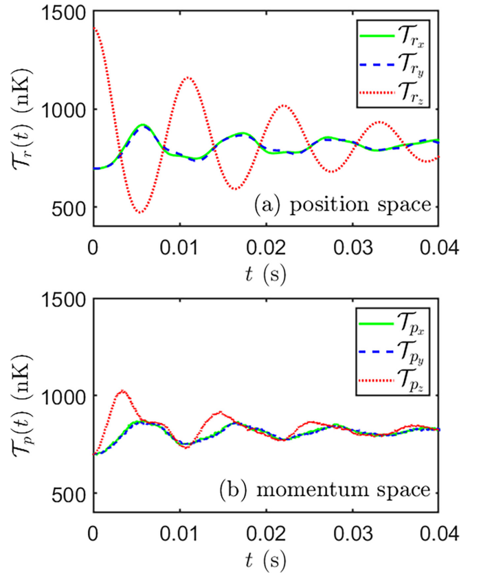
FIG. 2. Plots of the \mathcal{T}_i [upper panel (a)] and \mathcal{T}_{vi} [lower panel (b)] vs time from a cross-dimensional rethermalization experiment, with excitation along z . The gas is hydrodynamic with N = 5 \times 10^5 ( \text{Kn} \approx 0.04 ), \lambda = 0.2 and the parameters in Table I.
