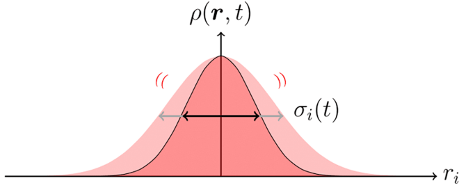
FIG. 4. Diagram of a density slice along axis r_i , through the Gaussian ansatz for \rho(\mathbf{r}, t) with time varying widths \sigma_i(t) .
