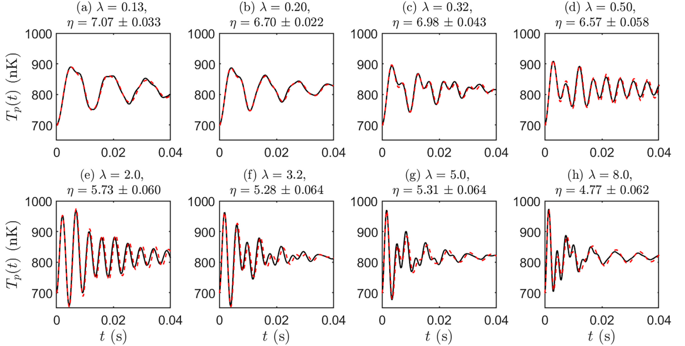
FIG. 6. Comparison of the momentum space temperature T_p (21) vs time t , obtained from DSMC simulations (black solid curves) and our theory (red dashed curves) with N = 5 \times 10^5 ( \text{Kn} \approx 0.04 ), \Theta = 90^\circ , and parameters in Table I. The subplots (a) to (h) correspond to various values of trapping anisotropy with \lambda = 0.13 to 8.0 as labeled in the subplot headers. The fitted values of \eta are also provided in the subplot headers with their fitting standard uncertainties.
