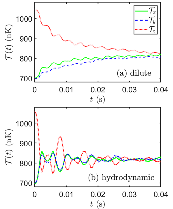
FIG. 1. Pseudotemperatures (2) obtained from Monte Carlo simulations in the dilute [upper panel, (a)] and hydrodynamic [lower panel, (b)] regimes. The gas consists of microwave shielded ^{23}\text{Na } ^{40}\text{K} molecules with dipole moment d = 0.75 D, oriented along \hat{x} , at temperature T = 700 nK. The gas is initially excited along z by an instantaneous trap frequency ramp to \omega_z = 2\pi \times 147 Hz, while \omega_x = \omega_y = 2\pi \times 82.5 Hz remain constant. The regimes are differentiated by the number of molecules N , which are N = 10^4 in panel (a), and N = 2 \times 10^5 in panel (b).
