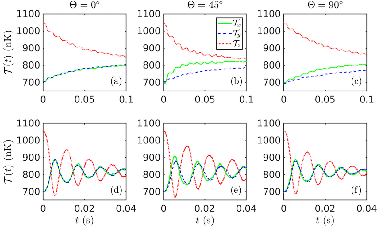
FIG. 3. Pseudotemperature times traces \mathcal{T}_x(t) (solid green curves), \mathcal{T}_y(t) (dashed blue curves), and \mathcal{T}_z(t) (dotted red curves) for the three values of \Theta = 0^\circ, 45^\circ, 90^\circ , in subplots (a,d), (b,e), and (c,f) respectively. The two rows are differentiated by the number of molecules, with the upper row [subplots (a)–(c)] having N = 2 \times 10^3 ( \text{Kn} \approx 11.10 ), while the lower row [subplots (d)–(f)] has N = 3 \times 10^5 ( \text{Kn} \approx 0.07 ). The experimental parameters are those in Table I with \lambda = 0.2 . Note that the simulation times are different between the upper ( t = 0 to 0.1 s) and lower ( t = 0 to 0.04 s) rows.
