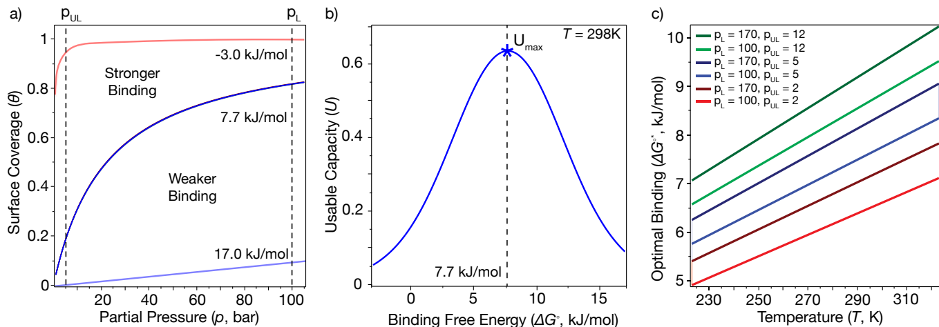
Fig. 2 An analysis of optimal binding interactions for high-density hydrogen storage on MOFs. The target H_2 standard binding free energy of a site optimizes the usable capacity ( U ) of a storage material, which (for given temperature, site density and either 0 or 1 H_2 per site) is proportional to the change in binding site occupancy (coverage, \theta ) between a high loading pressure (e.g. p_L = 100 bar in (a)) and a low unloading pressure (e.g. p_{UL} = 5 bar in (a)). (a) Binding isotherms for the Langmuir model for 3 different binding free energies at room temperature ( T = 298 K), illustrating the loss of usable capacity with too strong binding and too weak binding. (b) The dimensionless usable capacity U(T, p_L, p_{UL}) as a function of the standard free energy of binding at room temperature, for p_L = 100 bar, p_{UL} = 5 bar. (c) Optimal binding free energy \Delta G^{o*}(T) that correspond to U_{max} as a function of temperature for 6 different choices of the loading and unloading pressures p_L, p_{UL} .
