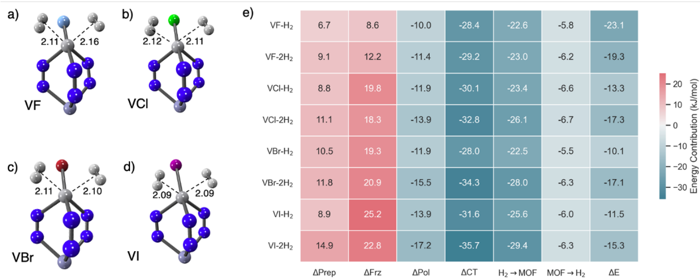
Fig. 13 Multiple H 2 ligations in V(II)-X-MFU-4l, (X = F, Cl, Br, I) (a-d) and EDA of the quite wide range of adsorption behaviour as a function of the halide counterion (e). Dative effects, particularly forward donation, dominate the binding energy. Distances are reported in Å, and energy contributions in kJ/mol in (e).
