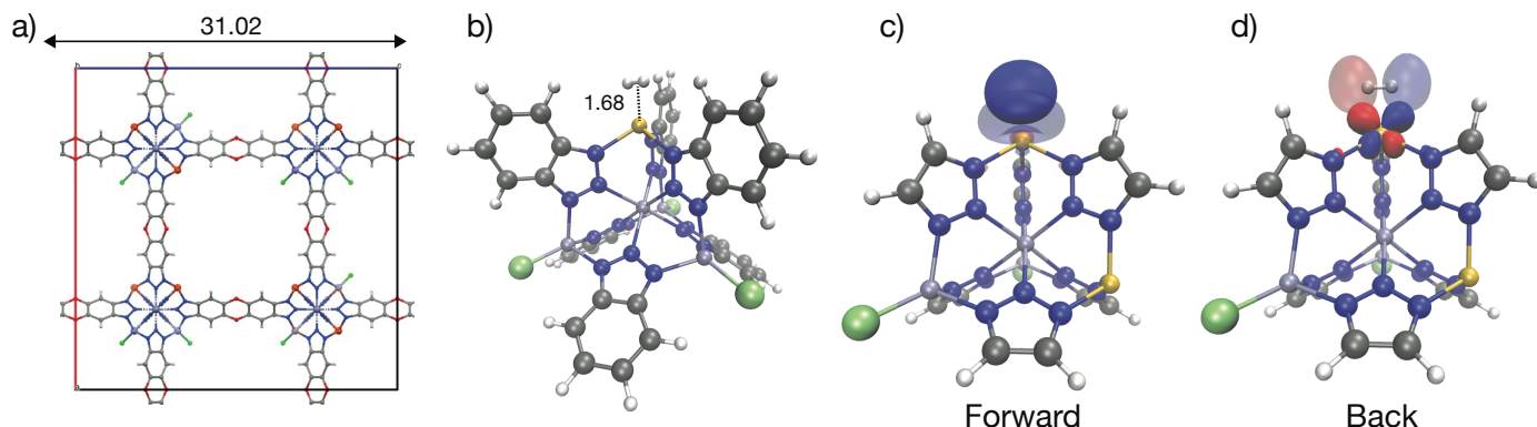
Fig. 7 Illustration of strong \text{H}_2 binding at the Cu(I) site in Cu(I)-MFU-4l. Panel (a) shows the cubic unit cell of the material, and (b) shows the cluster model representation \text{H}_2 binding in Cu(I)-MFU-4l; note the short 1.7 Å Cu– \text{H}_2 distance. Tetrahedral Cu(I) binding site with significant charge transfer orbitals for forward- and back-donation are shown in (c) and (d). Cu(I)– \text{H}_2 back-bonding interactions are strong at this binding site (see also Fig. 9). Distances are labelled in Å with Zn(II) rendered in blue-grey, Cu(I) in bronze, N in blue, H in light grey, C in dark grey, and Cl in light-green. The orbitals were plotted with an isosurface of \pm 0.07 Å. A smaller cluster model truncated at triazolate extremities was used for the visualization of charge transfer orbitals.
