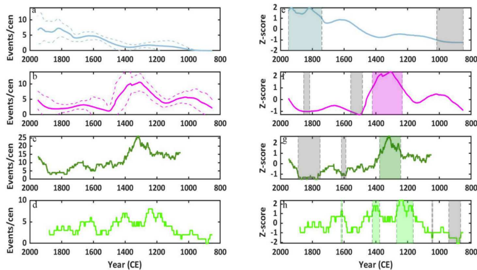
Fig. 5. (a) 100-yr frequency analysis for Pelican Cays composite record, (b) re-analyzed Northeast Yucatan composite record, (c) re-analyzed Great Blue Hole record (Denommee et al., 2014), and (d) re-analyzed Great Blue Hole record (Schmitt et al., 2020). (e–f) Moving Z-score derived from each respective 100-yr frequency analysis with colour-shaded regions indicating active intervals ( > +1\sigma ) and grey-shaded regions indicating quiet intervals ( < -1\sigma ). (For interpretation of the references to colour in this figure legend, the reader is referred to the web version of this article.)
