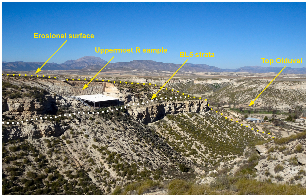
Picture 1. View of Barranco Leon site showing the location of the upper boundary of the Olduvai in the lower part of the Vélez Valley and the uppermost reverse paleomagnetic sample 5 m below an erosional surface.
