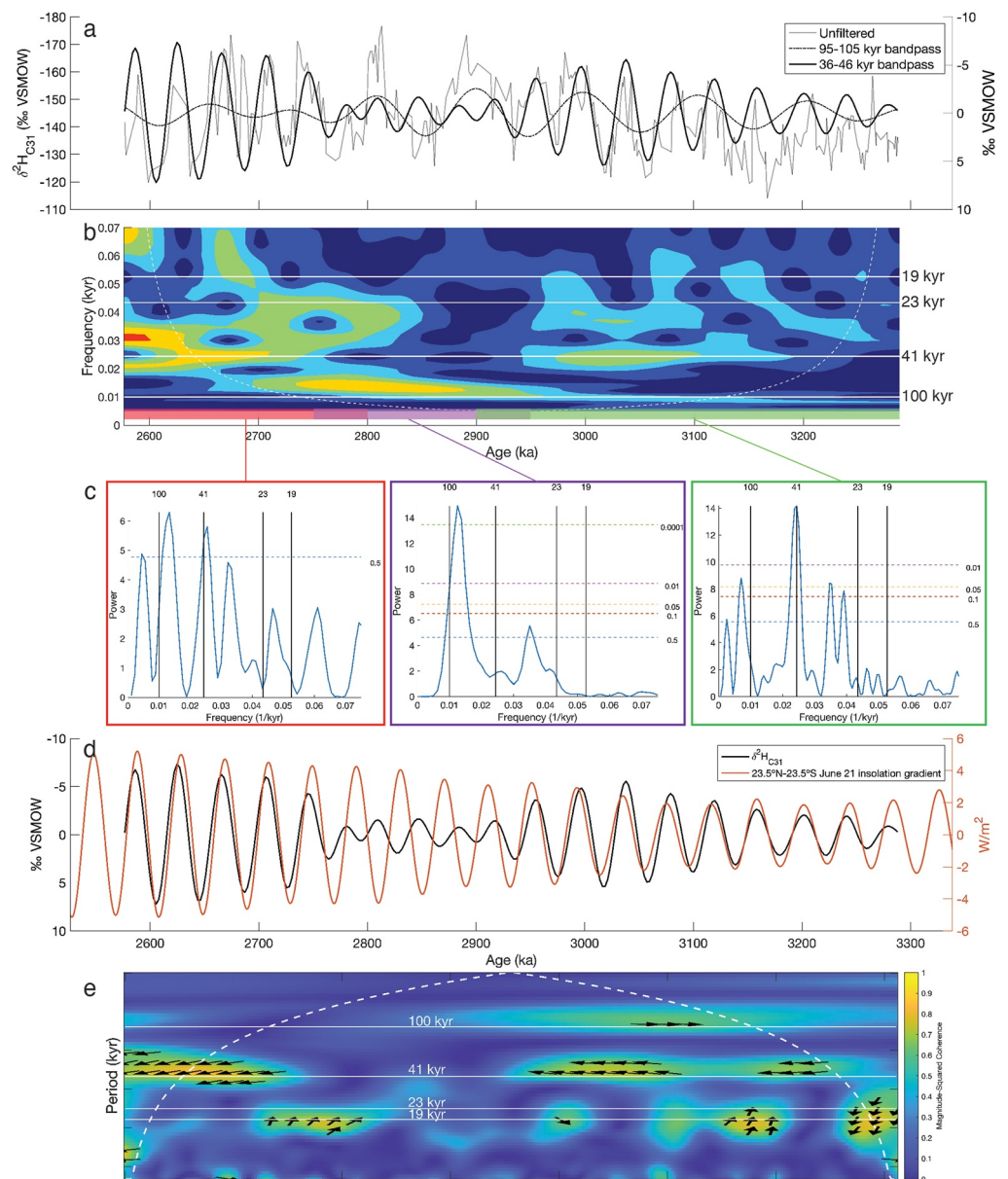
Figure 6. Spectral characteristics of the BTB13 \delta^2\text{H}_{\text{C31}} record. (a) Unfiltered (gray) and 36–46 kyr (black) and 95–105 kyr (dash-dotted) bandpass filtered \delta^2\text{H}_{\text{C31}} values. (b) \delta^2\text{H}_{\text{C31}} evolutionary wavelet power spectrum. Dashed white line denotes cone of influence. (c) Lomb-Scargle power spectra of 2.80–2.58 Ma (red), 2.95–2.75 Ma (purple), and 3.28–2.90 Ma (green) intervals. Dashed lines denote false alarm probability. (d) 36–46 kyr-bandpass filtered \delta^2\text{H}_{\text{C31}} values (black) and 21 June 23.5°N–23.5°S insolation gradient (orange). (e) Wavelet cross-spectrum of BTB13 \delta^2\text{H}_{\text{C31}} values and 21 June 23.5°N–23.5°S insolation gradient. Dashed white line denotes cone of influence. Arrows ( \geq 0.60 magnitude-squared coherence) pointing to the left indicate 0° phase lead/lag.
