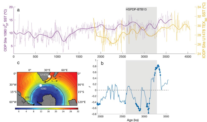
Figure 8. (a) Sea surface temperatures (SSTs) from ODP Site 1090 ( U^{k'}_{37} ) (Martínez-García et al., 2010) (purple) and International Ocean Drilling Program Site U1478 ( TEX_{86} ) (Taylor et al., 2021) (gold). (b) A running 10-point Pearson's r of Site 1090 and U1478 SSTs. Filled circles indicate intervals where correlation is statistically significant ( p \leq 0.05 ). Shading indicates the timespan of BTB13. (c) Locations of Sites 1090 and U1478, the modern-day subtropical front (Orsi et al., 1995), and the Agulhas leakage (thick arrow) and retroflection/return current (dashed arrows) (Bard & Rickaby, 2009; Graham & De Boer, 2013). Background is 0.25^\circ \times 0.25^\circ gridded 1982–2010 average SSTs (Reynolds et al., 2007).
