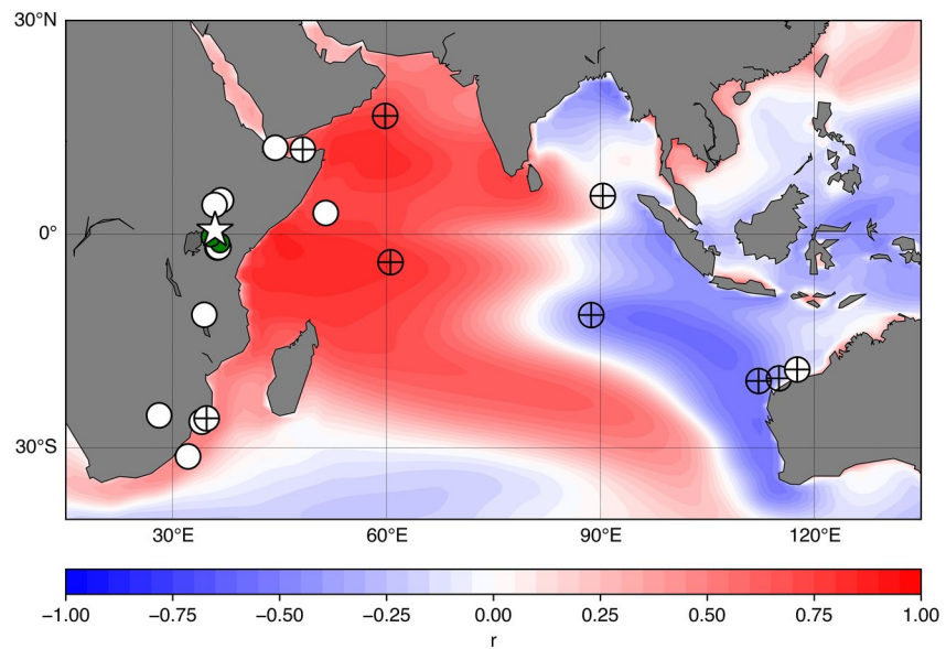
Figure 1. Locations of Kenyan Global Network of Isotopes in Precipitation stations (green), HSPDP-BTB13-1A (white star), and other Pliocene-Holocene terrestrial hydroclimate (white circle) and sea surface temperature (SST) records (cross). Background is annual field correlations ( r ) between an 1,800-year preindustrial control run of CESM1 SSTs and mean annual eastern African rainfall (averaged over -5.183 – 7.068^\circ\text{N} and 35 – 46.25^\circ\text{E} ) (Tierney et al., 2013). See Table 1 and Figure 4 for site names.
