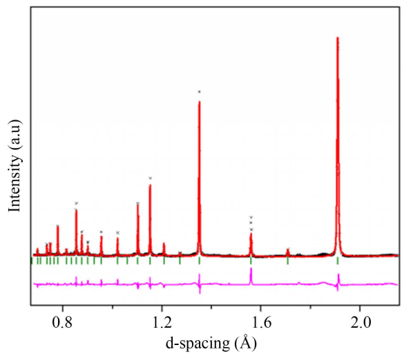
Figure 3. Neutron diffraction Rietveld refinement profile. Crosses represent experimental data, the solid red line is the Pm-3m model, vertical green tick marks show Bragg peak positions, and the lower pink line represents the difference plot.
