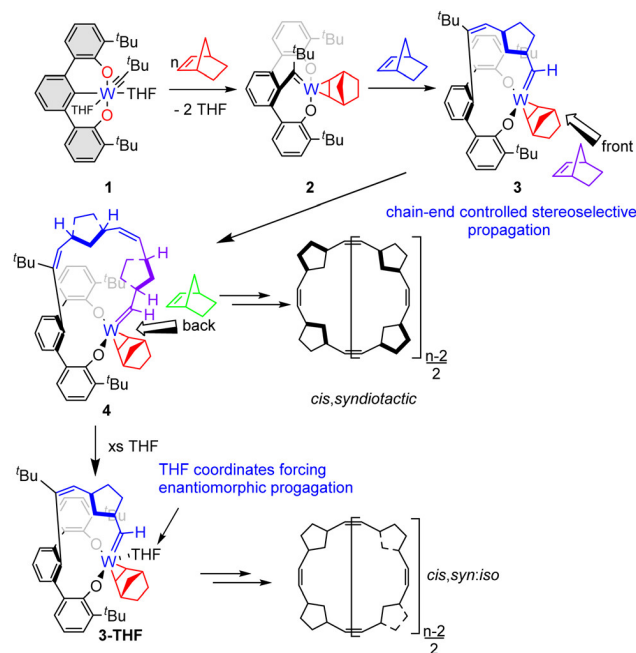
Scheme 2 Proposed initiation and role of THF in REMP of norbornene with 1 . In toluene both enantiofaces are open allowing norbornene to approach alternating faces creating syndiotactic PNB. In THF, one enantioface is blocked forcing approach at the same face creating isotactic blocks.
