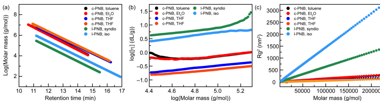
Fig. 1 (a) Log of molar mass versus elution time (b) log of intrinsic viscosity ( [\eta] ) versus log of molar mass, and (c) mean square radius ( R_g^2 ) versus molar mass for c-PNBs synthesized by 1 in various solvent and l-PNBs.
