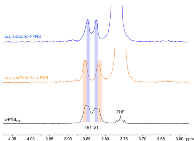
Fig. 3 H(1',6') signal with homonuclear decoupling at 2.61 ppm in the 1 H NMR spectra of partially brominated cis, syndiotactic -l-PNB (orange) and cis, isotactic -l-PNB (blue), and c-PNB synthesized by 1 in THF. Note: isotactic H(1',6')s are two unresolved doublets with 2.5 Hz coupling, thus appearing as a singlet.
