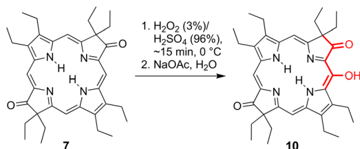
Scheme 5 Synthesis of 5-hydroxy-7,17-dioxobacteriochlorin 10 by oxidation of the parent 7,17-dioxobacteriochlorin 7 .
