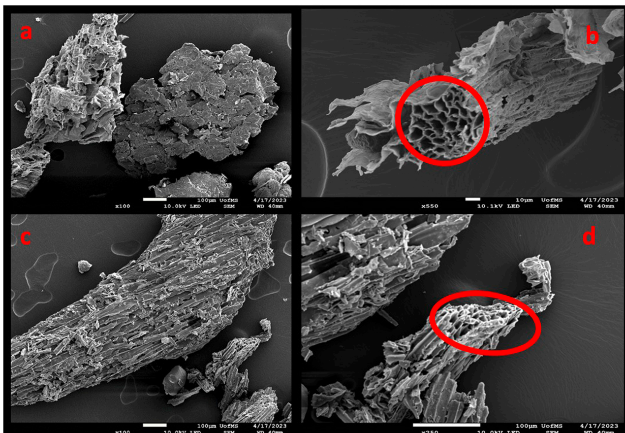
FIGURE 5 SEM images of sugarcane biochar (A,B) and pinewood biochar (C,D) showing rough surface features and pores (circled in red). Images at 100 × magnification (A,C), 250 × magnification (D), and 550 × magnification (B).
