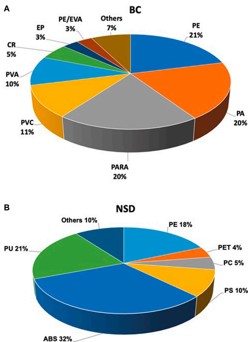
FIGURE 3 Distribution (%) of microplastics by type in BC (A) and NSD (B) sample sites ( n = 2 per site) in agricultural runoff at a farm in the Mississippi Delta. Acronyms not previously defined: CR, crumb rubber; EVA, ethylene vinyl acetate; PVA, polyvinyl alcohol; EP, ethylene propylene rubber; PU, polyurethane; PS, polystyrene.
