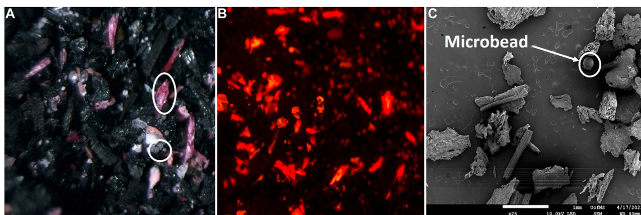
FIGURE 6 Representative microscopy images of Pinewood biochar column fraction containing microplastics (LDPE, PA, PET, PC, PS, PE, PVC): optical (A), fluorescence (B), and SEM (C). All images are from the same Pinewood biochar column fraction.
