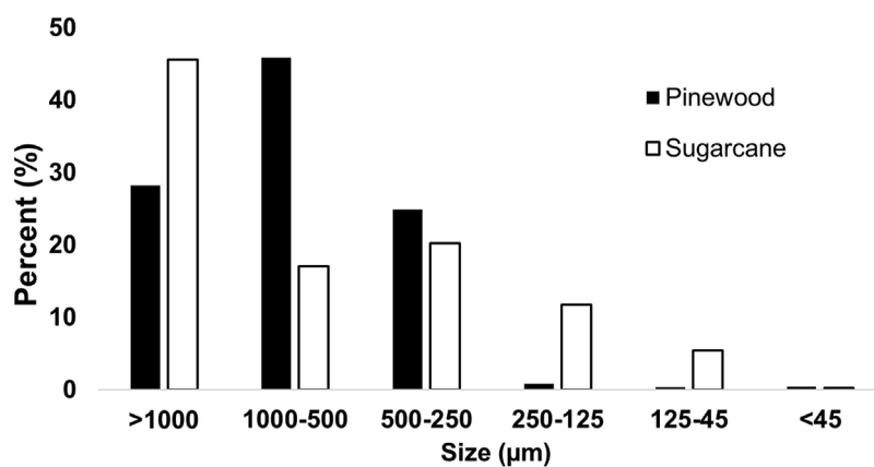
FIGURE 4 Particle size distribution (percent by mass) of pinewood and sugarcane biochar.
