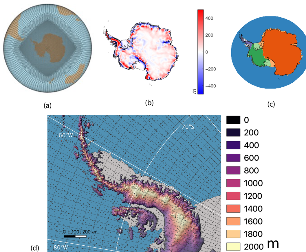
Figure 1. Elevation on (a) the ANTISI grid with 0.25^\circ spectral element points in the interior and 1^\circ in the exterior. (b) Difference between interpolated surface elevation (ANTISI-AMIP) (c) regions shown for East Antarctica (orange), West Antarctica (green), and the Antarctic Peninsula (purple), with lighter shades indicating ice shelves and darker shades indicating the grounded ice sheet; from Zwally et al. (2002). (d) Elevation (source: ETOPO) with the AMIP grid shown by lines and ANTISI spectral element points shown as dots over the Antarctic Peninsula.
