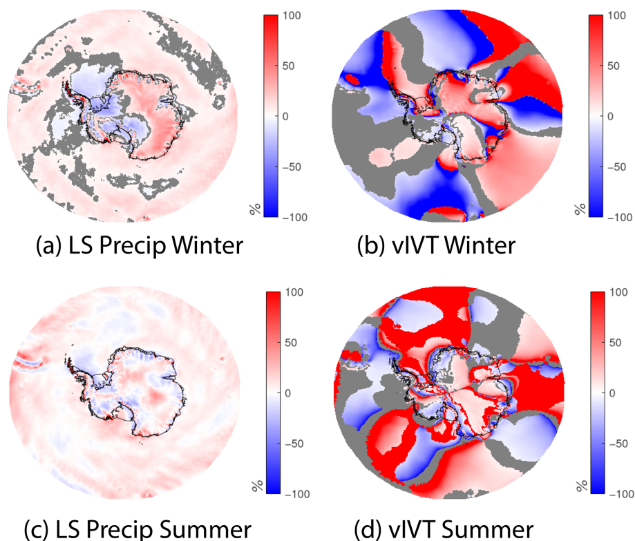
Figure 6. Relative change (%) in large-scale (LS) precipitation and integrated meridional vapor transport (vIVT) between ANTISI and AMIP for the 1979–2014 seasonal mean (grey indicates where biases are not significant compared to the AMIP ensemble SD). (a) Large-scale precipitation for winter (JJA) and (c) summer (DJF). Integrated meridional vapor transport for winter (b) and summer (d).
