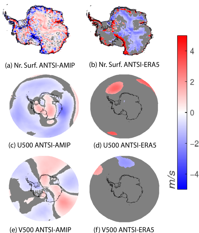
Figure 10. Mean winter (JJA) wind speed differences (1979–2014) between ANTISI-AMIP (a, c, e) and ANTISI-ERA5 (b, d, f) for the near surface (a, b), the 500 hPa zonal component (c, d), and the 500 hPa meridional component (e, f). Grey indicates where biases are not significant compared to the AMIP ensemble SD.
