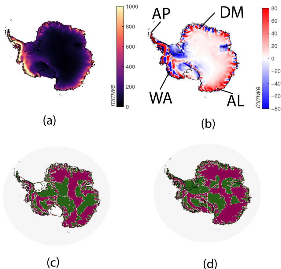
Figure 3. Surface mass balance (SMB) over the 1979–2014 period. (a) SMB from ANTISI; (b) difference in SMB (ANTSI–AMIP). Regions indicated include the Antarctic Peninsula (AP), Dronning Maud Land (DM), West Antarctica (WA), and Adélie Land (AL). Panels (c) and (d) show ANTISI SMB bias relative to AMIP compared to the reconstruction and RACM2.3, with green and purple indicating reduced or increased bias in ANTISI relative to the dataset.
