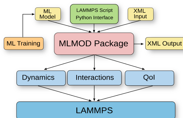
Figure 2: The MLMOD Package is structured modularly with subcomponents for providing ML models in simulations for the dynamics, interactions, and computing quantities of interest (Qol) characterizing the system state. The package makes use of standardized data formats such as XML for inputs and export ML model formats from machine learning frameworks.
