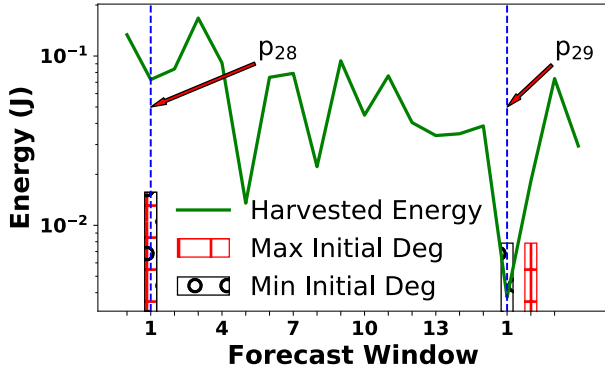
Fig. 3: Degradation influence.
