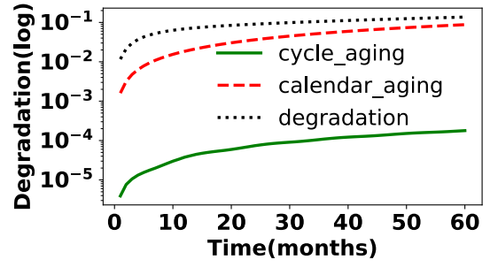
Fig. 2: Battery degradation.
