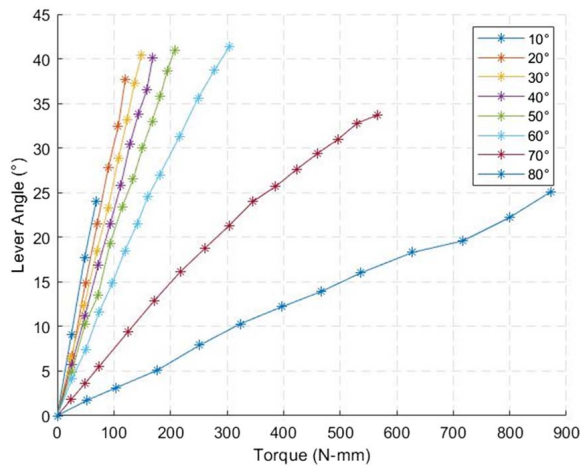
Fig. 14 Testing results for antagonistic mechanism
