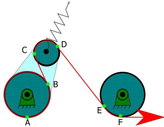
Fig. 5 Cable length segments
