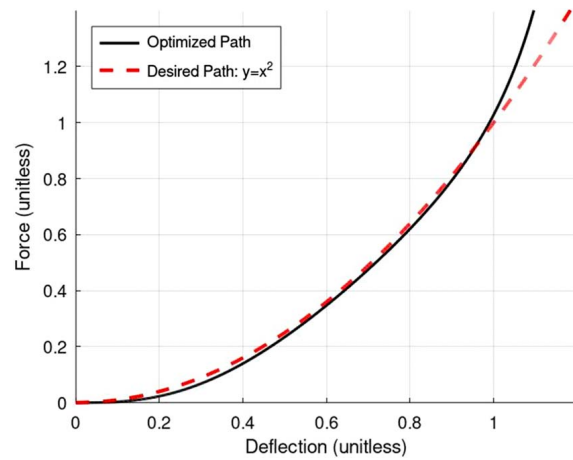
Fig. 8 Final mechanism force-deflection curve
