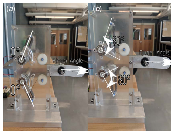
Fig. 13 Stiffness configuration examples
