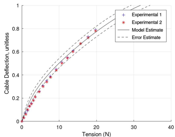
Fig. 12 Testing results for single-sided mechanism
