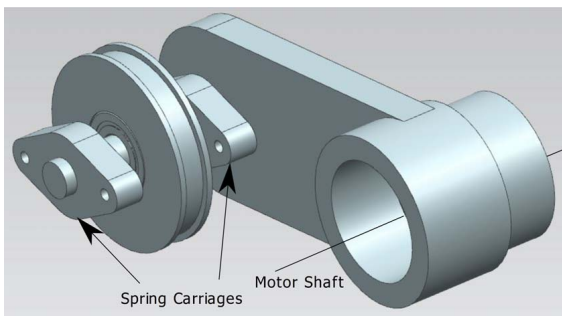
Fig. 11 Lever shaft assembly and spring carriage
