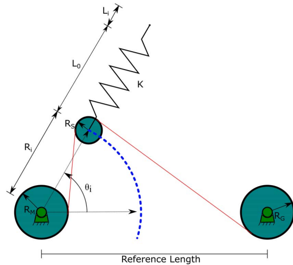
Fig. 6 Mechanism design parameters
