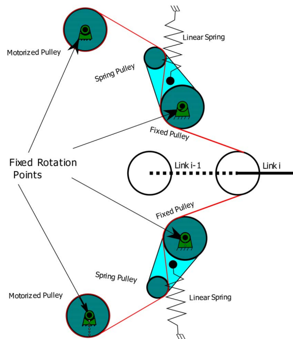
Fig. 1 DLR's flexible antagonistic spring element design
