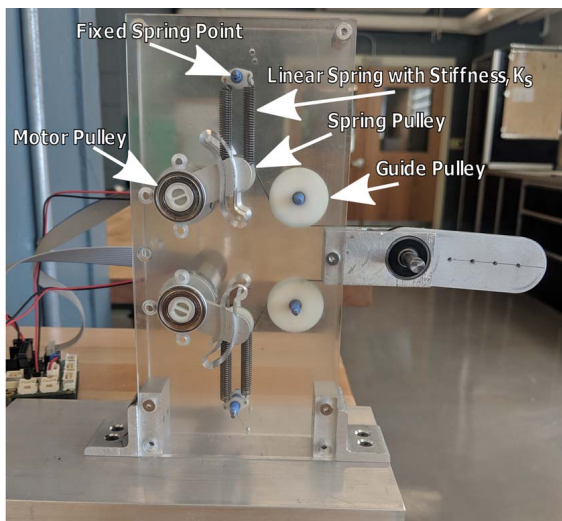
Fig. 10 Testing apparatus for VSA
