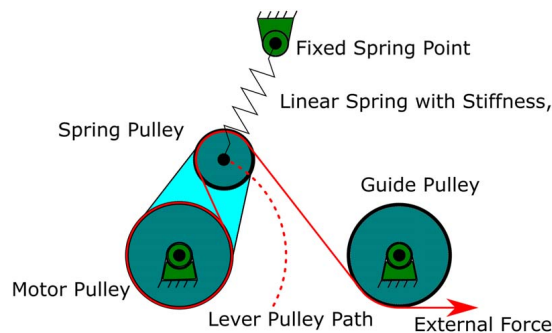
Fig. 2 One side of the antagonistic, quadratic stiffness cable-driven VSA design
