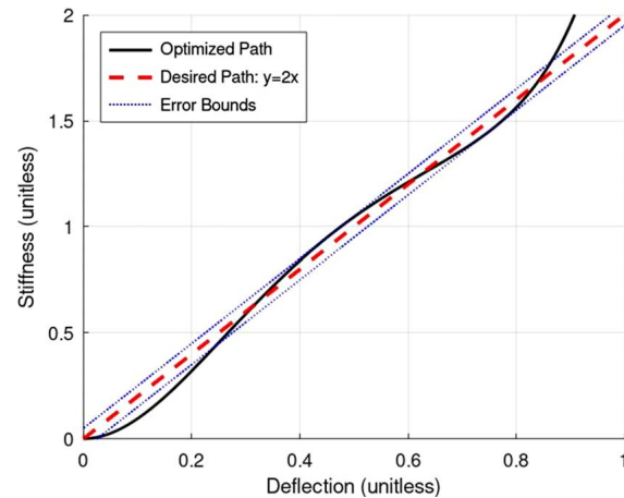
Fig. 9 Final mechanism stiffness-deflection curve
