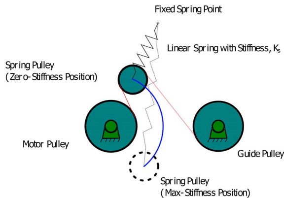
Fig. 7 Final mechanism configuration
