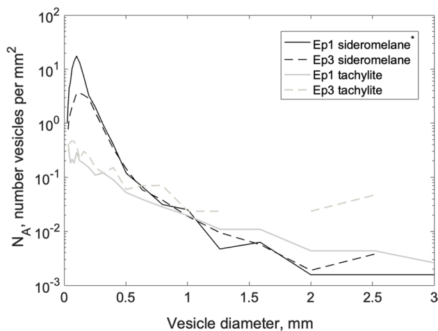
Fig. 9 Vesicles per unit area ( N_A ) for sideromelane from episode 1 (Stovall et al. 2011) and episode 3 (sample KI06-13–14-T17) and tachylite from episode 1 (sample KI07-07-p11-Tv1) and episode 3 (KI06-13–14-T17). The plots are generated by combining three hierarchies of data: the optical scan number densities are used for vesicle size bins >0.5 mm; and data from two nested SEM images (with pixel sizes of 12 and 7 \mu\text{m} ) for bin sizes 0.25–0.4 mm and <0.25 mm respectively, after Stovall et al. (2011)
