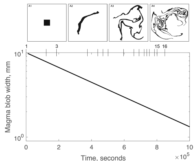
Fig. 11 Top, the process of progressive stretching and folding of magma blobs within another magma host is proposed to produce commonly observed magma mingling textures (sketches at the top from Petrelli et al. 2011). Bottom, the application of a simple dimensionless model to understand how the width of an entrained magma blob may decrease with time during chaotic magma flow shows that, when translated to real dimensions the width of a 10-mm blob can decrease to \sim 1 mm over around 10^6 s, or \sim 12 days. The timings of episodes 1–16 are marked on the top of the plot; episodes 1, 3, 15, and 16 are labelled (see text for the detail of the model)
