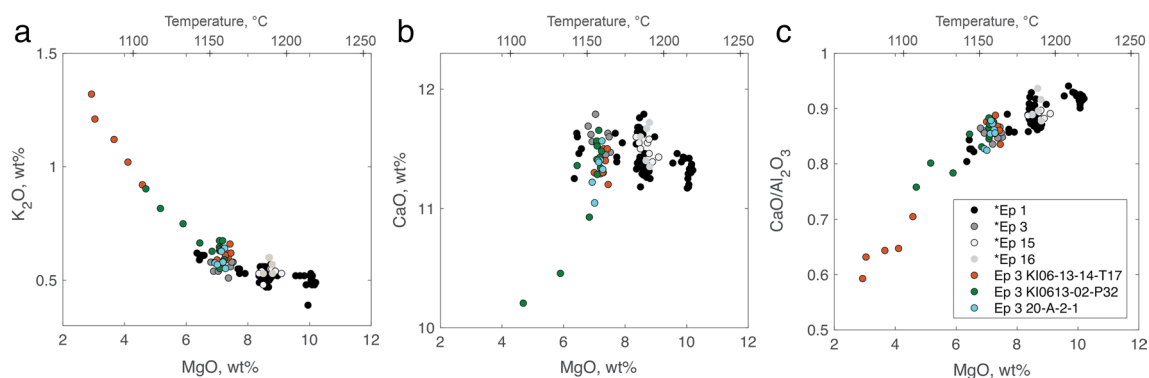
Fig. 6 Electron microprobe data for glasses in three episode 3 samples: KI06-13-14-T17, KI06-13-02-P32, and 20-A-2-1. Plots show MgO (wt%) versus K 2 O (wt%) ( a ); CaO (wt%) ( b ); and CaO/Al 2 O 3 ( c ), showing a tight cluster of sideromelane glasses at ~7.2 ± 0.4
