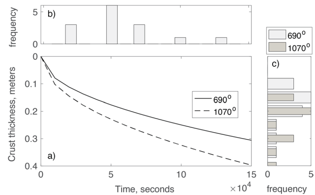
Fig. 10 a A thermal model to predict the thickness of a lava lake crust with base temperatures of 690 and 1070 ^{\circ}\text{C} with time, based on the balance between conductive heat loss to the upper layer of the lake and latent heat of crystallisation (Worster et al. 1993) in a crust at the top of the lava lake. In b and c , we show the frequency distribution of repose times between episodes ( x axis as in a ), and crust thicknesses calculated using repose times and thermal model, respectively, ( y axis as in a )
