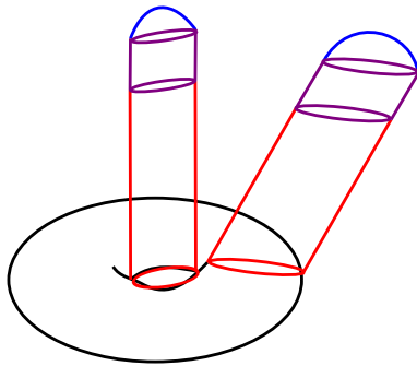
Figure 6. An image of the Liouville-sectorial cover of the Weinstein manifold obtained by gluing in disks along circles in homology classes (1, 0) and (0, 1) . The three pieces in the cover are the torus with cylinders attached; a pair of disks; and their intersection, a pair of cylinders.
