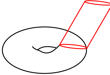
Figure 4. The skeleton \mathbb{L}_\Sigma for \Sigma the fan of \mathbb{C} \times \mathbb{C}^\times , given as the union of a torus (in black) with a cylinder (in red).
