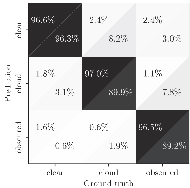
Figure 14. The confusion matrix of the CNN classifier. The numbers in the diagonal (off-diagonal) blocks are the true-positive (true-negative) rate for each column. The two values in each block correspond to the statistics for daytime (upper left) and nighttime (lower right).
