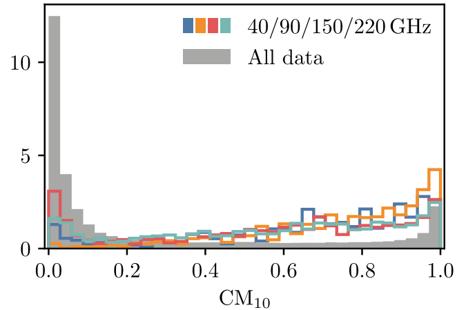
Figure 9. The distribution of cloud measure above 10^\circ elevation ( CM_{10} ) associated with each of the CLASS polarization detections. The colored histograms correspond to the polarization detections from each of the four frequencies. The global CM_{10} distribution from all data is shown in gray.
