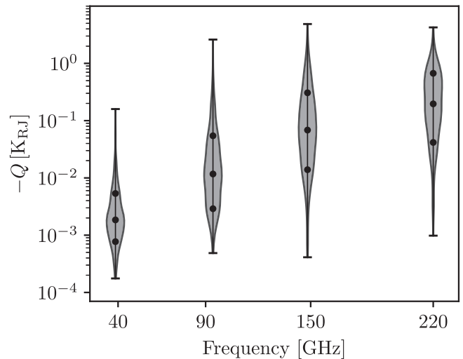
Figure 11. Measured cloud polarization signal ( -Q ) as a function of the effective frequency. The samples include all 90 GHz-selected candidates with an S/N > 4 at each band. The dots mark for each distribution the 16, 50, and 84 percentiles.
