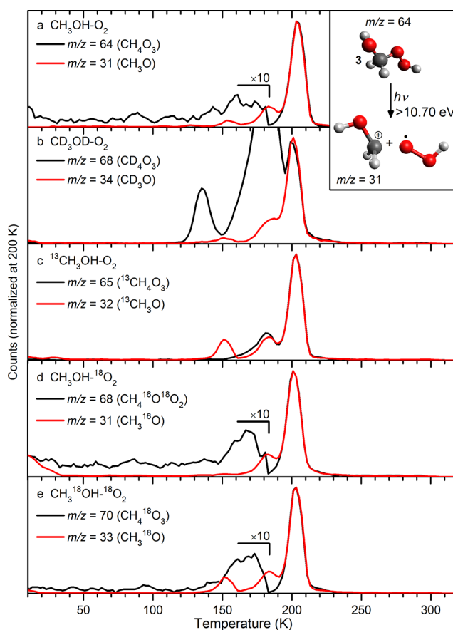
Figure 6. The 10.86 eV photoionization TPD profiles of isotopomers of \text{CH}_4\text{O}_3^+ and \text{CH}_3\text{O}^+ . These TPD profiles are all shown after normalization of the peak at 200 K. This peak is observed for all studied isotopomers of \text{CH}_4\text{O}_3^+ , confirming the assignment of this molecular formula. The peak at 170 K is observed without obstruction in both \text{CH}_3\text{OH}-^{18}\text{O}_2 and \text{CH}_3^{18}\text{OH}-^{18}\text{O}_2 ices. Furthermore, the consistent match of this peak with \text{CH}_3\text{O}^+ shows that this sublimation event is accompanied by fragmentation of the specific isomer of \text{CH}_4\text{O}_3^+ upon sublimation at 200 K.
