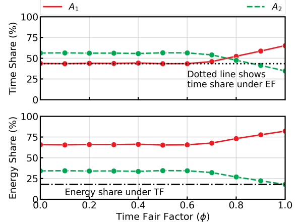
Figure 11: Energy and time allocations under ETF at varying values of \phi . A_1 runs ResNet50 at 1300 MHz and A_2 runs MobileNet-V2 at 726 MHz with weights 2-to-1.
