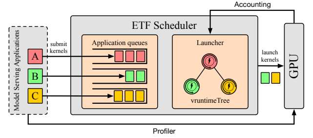
Figure 4: Architecture of ETF implementation.
