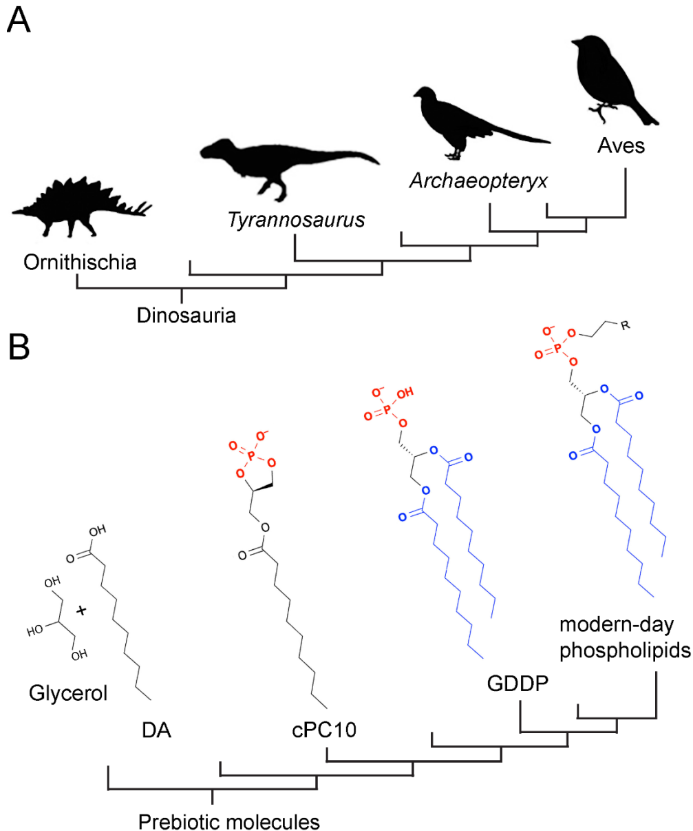
Figure 1. Illustrations of transitional forms in animal evolution and proposed prebiotic membrane evolution. (A) Archaeopteryx and Tyrannosaurus are among the transitional forms found in the fossil record characterizing the evolution of modern birds (Aves) from dinosaurs (adapted from ref. 8 ). (B) Cyclic-phospholipids such as cPC10 are produced from fatty acid (e.g., decanoic acid (DA)) and glycerol with phosphorylation with DAP. The hydrolysis of the cyclic phosphate moiety followed by esterification leads to diacyl-phospholipids (GDDPs), whose modification would produce modern phospholipids.
