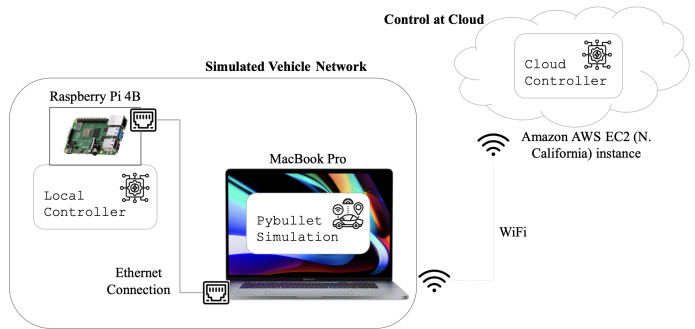
Fig. 2: System Setup
