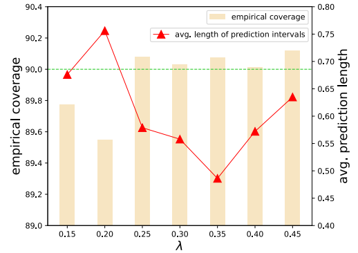
Figure 2: Performance of S-CQR for conformalized link prediction under different \lambda on Rochester38 dataset.
