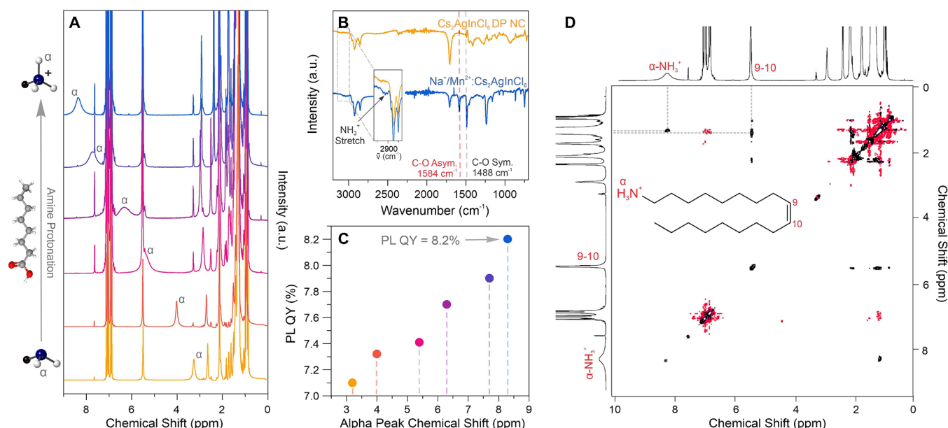
Figure 4. (A) 1 H NMR spectra of the Na + /Mn 2+ codoped Cs 2 AgInCl 6 DP NC solutions following the protonation of OAm (bottom) to form oleylammonium (top). (B) FTIR spectra of the as-synthesized Cs 2 AgInCl 6 DP NCs (orange) and Na + /Mn 2+ codoped Cs 2 AgInCl 6 DP NCs (blue). (C) Correlated PL QY increased with the increased level of OAm protonation (oleylammonium formation). (D) 2D-NOESY spectrum of the Na + /Mn 2+ codoped Cs 2 AgInCl 6 DP NCs. The black and red signals represent the positive and negative cross-relaxation rates, respectively.
