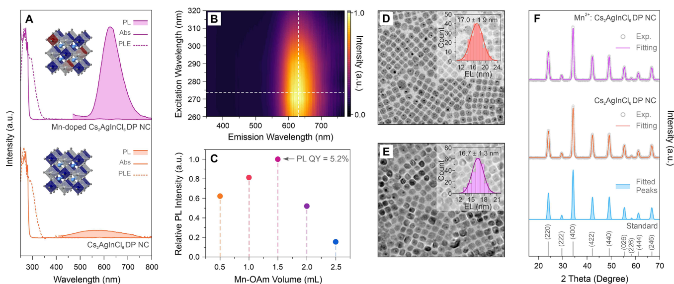
Figure 1. (A) Absorption spectra (solid lines), PLE spectra monitored at the strongest PL peak (dashed lines), and PL spectra (solid lines with shading) of the as-synthesized Cs 2 AgInCl 6 DP NCs (orange) and Mn 2+ -doped Cs 2 AgInCl 6 DP NCs. (B) PL emission contour map of Mn 2+ -doped Cs 2 AgInCl 6 DP NCs. (C) Mn-OAm concentration-dependent PL intensity. (D, E) TEM images and size distribution histograms (insets) for the undoped (D) and Mn 2+ -doped DP NCs (E). (F) XRD patterns (gray open circles) and fitted patterns (solid lines) for the as-synthesized Cs 2 AgInCl 6 DP NCs (orange) and Mn 2+ -doped Cs 2 AgInCl 6 DP NCs (purple). Gray bars indicate the standard peak positions of bulk Cs 2 AgInCl 6 DP. The constituent fitted XRD peaks are shown in light blue.
