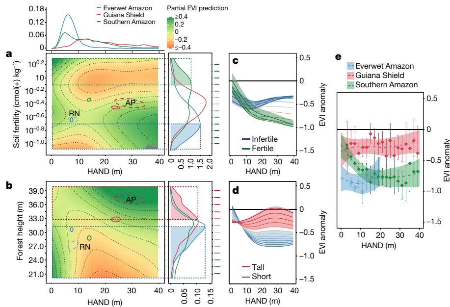
Fig. 4 | Basin-wide Amazon forest responses to the 2015 drought, structured by ecotopes and predicted by whole-basin GAM analysis. a, b , GAM partial predictions of EVI anomalies (colour scale) for soil fertility 43 (vertical axis) and HAND 25 (horizontal axis) terms only ( a ), and for forest height 45 and HAND 25 terms only ( b ). Ecotope distributions in southern, everwet and Guiana Shield forests ( a , top right and b , right), and associated 99% confidence ellipses (main graph). The mean values of two areas exhibiting green-up in Fig. 1c (RN, in Rio Negro catchment, and AP in Amapa state) illustrate differing mechanisms of green-up (especially evident in b , where tall trees, despite deep water tables, promote green-up in AP, while shallow water tables promote green-up for RN). c, d , Adjusted EVI anomaly versus HAND with increasing fertility (blue to green
