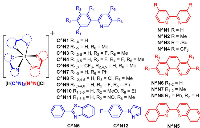
Fig. 9 Structures of photocatalysts used in experiment 2. Each complex contains two cyclometallating C AN ligands and one ancillary N AN ligand. All complexes have a Cl − counterion.
