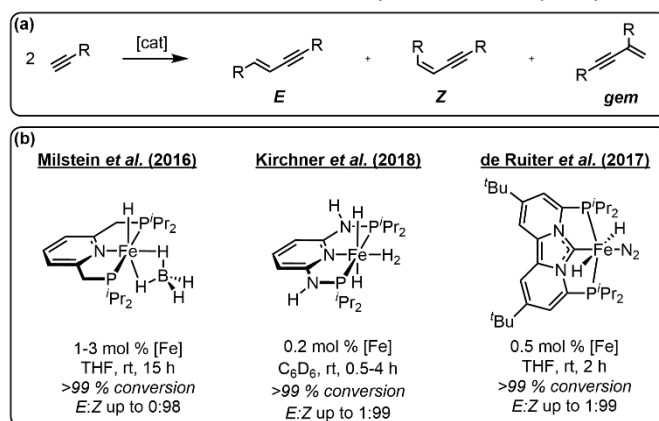
Fig. 1: (a) Possible 1,3-enynes resulting from the dimerization of terminal alkynes. (b) Selected examples of Z -selective homogeneous Fe-based (pre)catalysts for the dimerization of terminal alkynes
