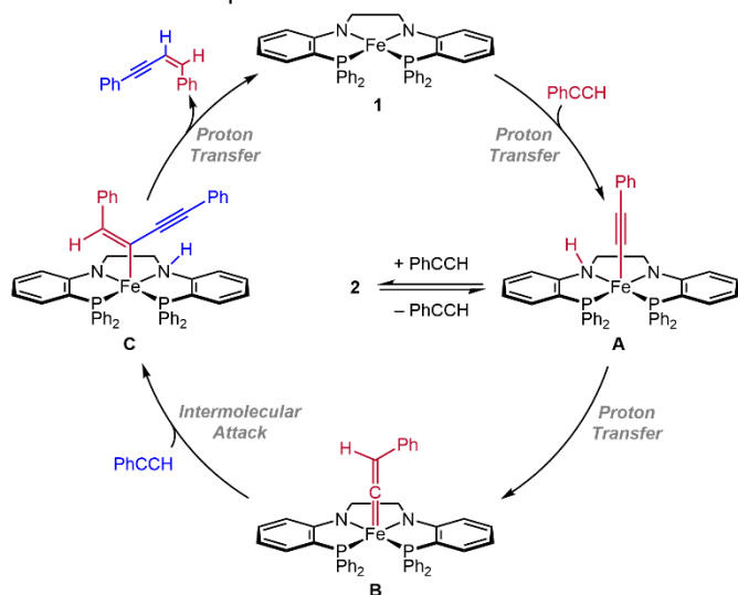
Fig. 1: Proposed catalytic cycle of alkyne dimerization by 1 .
