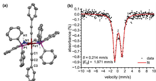
Fig. 2: (a) Displacement ellipsoid (50%) representation of 2 . For clarity, carbon-bonded H atoms and fluorobenzene solvent molecules are omitted, and symmetry-equivalent positions of the asymmetric unit are shown to provide a complete molecular representation. Relevant interatomic distances (Å) and angles (°): Fe1–P1: 2.1750(4), Fe1–N1: 2.0563(12), Fe1–C1: 1.9322(15), C1–C2: 1.219(2), C1–Fe1–C1': 171.38(9), Fe1–C1–C2: 171.45(13), C1–C2–C3: 175.97(16). (b) Fitted zero-field 57 Fe Mössbauer spectrum of 2 at 4 K.
