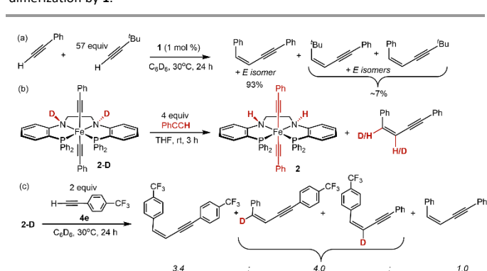
Scheme 2. Experiments performed to probe the mechanism of alkyne dimerization by 1 .
