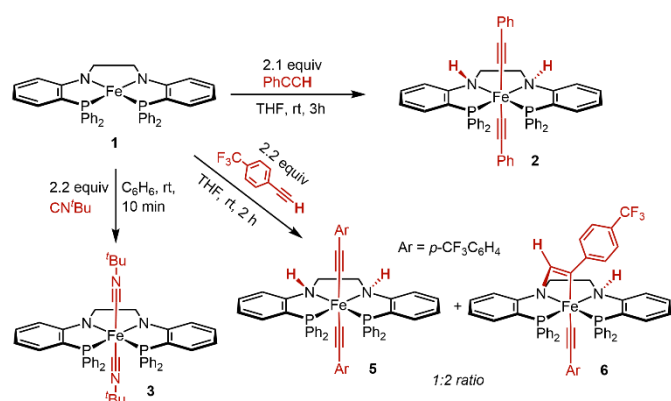
Scheme 1: Reaction of 1 with phenylacetylene, p-trifluoromethylphenylacetylene, and CN t Bu.
