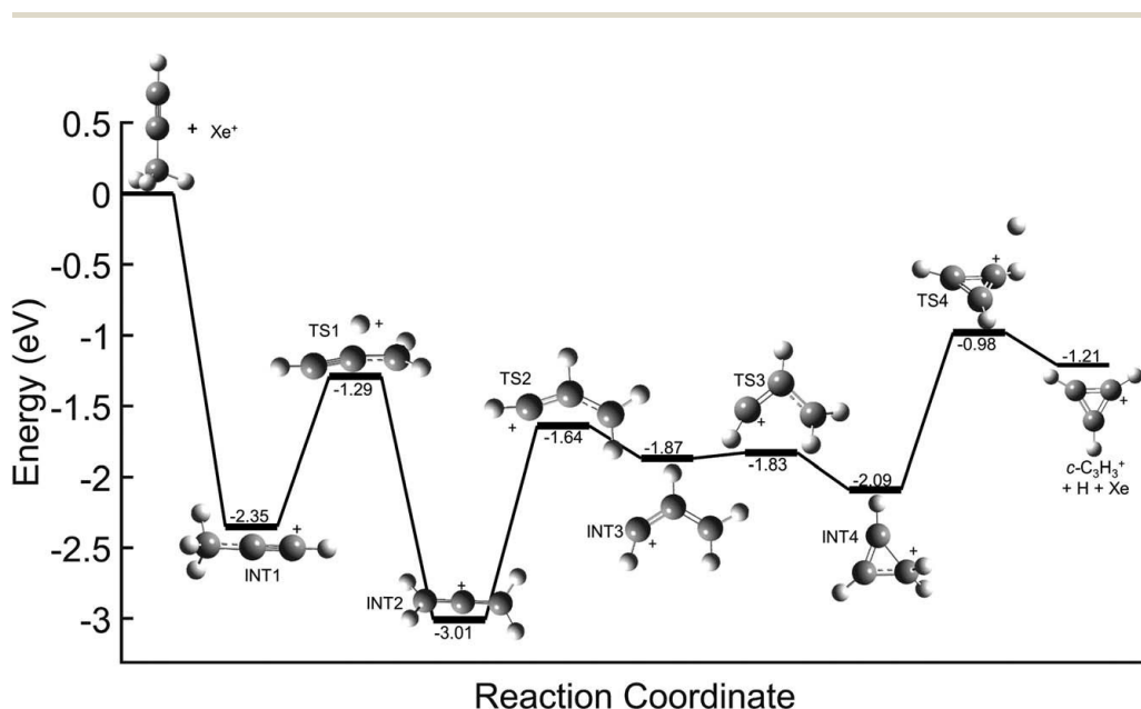
Fig. 6 Global potential energy surface of the reaction between \text{Xe}^+ and propyne ( \text{H}_3\text{C}_3\text{H} ) calculated at the \omega\text{b97x/aug-cc-pvtz} level. All energies are shown relative to reactant energy at infinite separation, with INT1 corresponding to the first stationary point following charge transfer. Note that the allene ( \text{H}_2\text{C}_3\text{H}_2 ) cation is identified as INT2, and the PES for allene with \text{Xe}^+ is identical to that shown here with energies being shifted to higher energies by 5 meV.
