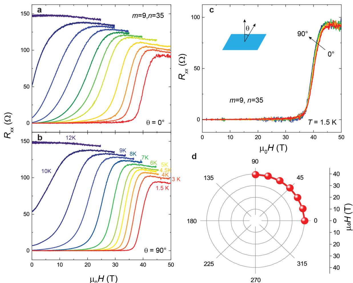
Figure 5. | Large and isotropic upper critical magnetic field in \text{MnBi}_2\text{Te}_4/\text{FeTe} heterostructures. a, b, R_{xx} - \mu_0H curves of the (9, 35) heterostructure under different T (a) \theta = 0^\circ (i.e., out-of-plane) and (b) \theta = 90^\circ (i.e., in-plane). c, R_{xx} - \mu_0H curves of the same (9, 35) heterostructure at T = 1.5 K under different \theta . Inset shows the angle \theta between the normal direction of the film and the magnetic field \mu_0H direction. d, \theta dependence of the upper critical magnetic field \mu_0H_{c2} . The value of \mu_0H_{c2} is determined as the magnetic field at which R_{xx} drops to \sim 50\% of its normal state value.
