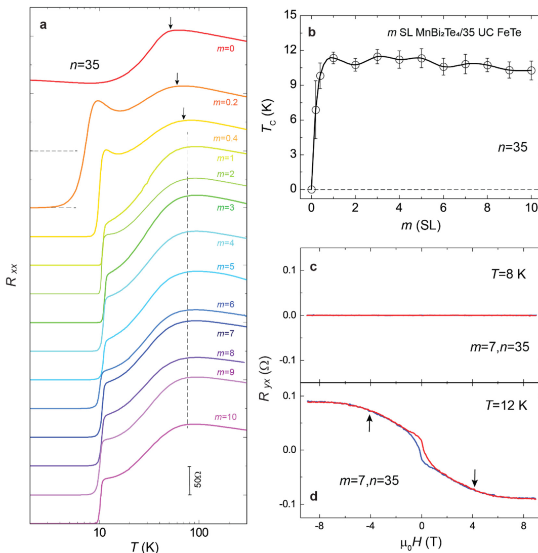
Figure 2. | Interface-induced superconductivity in \text{MnBi}_2\text{Te}_4/\text{FeTe} heterostructures. a, Temperature dependence of the sheet longitudinal resistance R_{xx} of the (m, 35) heterostructures with 0 \leq m \leq 10 . The two horizontal dashed lines represent zero resistance in the m = 0 and m = 0.2 heterostructures. The three arrows and the vertical dashed lines indicate the hump features resulting from the paramagnetic-to-antiferromagnetic phase transition. b, m dependence of the superconducting temperature T_c . The value of T_c is defined as the temperature at which R_{xx} drops to 50% of its normal state resistance. The error bar of each sample is estimated from the value difference between T_{c, \text{onset}} and T_{c, 0} . c, d, \mu_0 H dependence of the Hall resistance R_{yx} of the (7, 35) heterostructure at T = 8 K (c) and T = 12 K (d). The arrows in (d) mark the kink features associated with the spin-flop transition.
