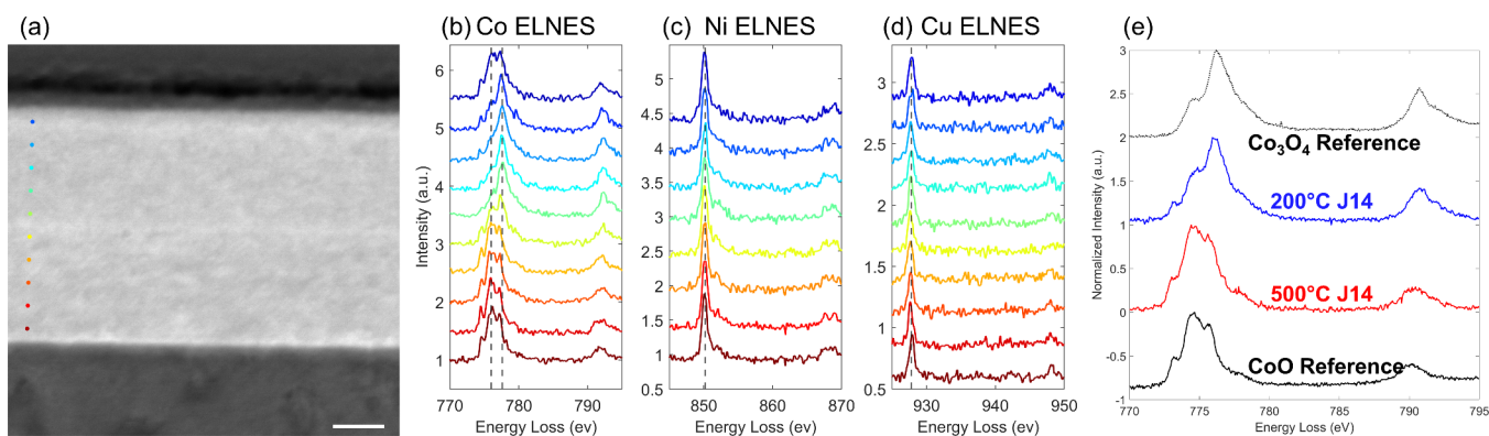
Figure 5. Line-scan monochromated STEM-EELS of 3d transition metal L edge energy loss near edge structure (ELNES). (a) Probe positions overlaid over the ADF-STEM image. Scale bar is 20 nm. (b–d) L edge ELNES for Co, Ni, and Cu, respectively. (e) Comparison between the averaged spectra from 200 °C J14 film, 500 °C J14 film, CoO reference spectra, and Co 3 O 4 reference spectra.
