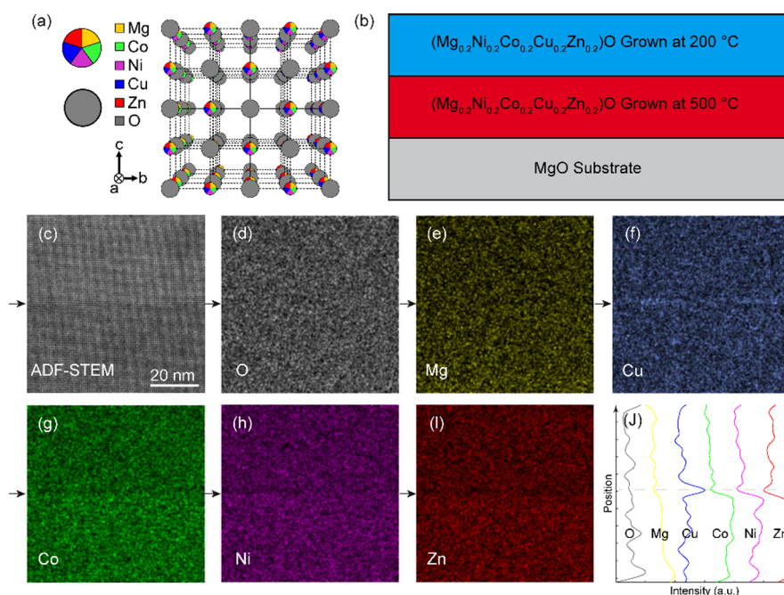
Figure 1. (a) Crystal structure model for the rocksalt structure HEO ( \text{Mg}_{0.2} , \text{Co}_{0.2} , \text{Ni}_{0.2} , \text{Cu}_{0.2} , \text{Zn}_{0.2} ) O viewing from the [100] axis; (b) schematics of the stacked HEO thin film synthesized with the PLD method; (c) high-resolution HAADF-STEM micrograph acquired at the interface of the stacked thin film, and (d–l) EDX map of the constituent elements taken at the same region as the HAADF-STEM micrograph in panel (c). The EDX maps are plotted with Gaussian filtering with filter size of 2 pixels. The interface between the stacked films is marked by the arrows. (j) Line-averaged EDX intensity profile with the interface location is marked by the dashed line.
