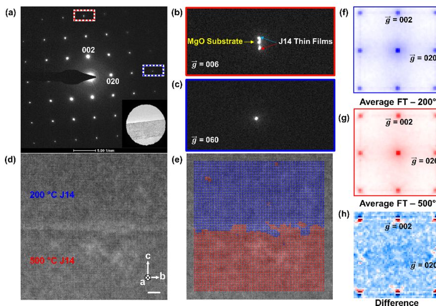
Figure 2. Reciprocal space investigation and the local crystallography analysis. (a) SAED pattern acquired from the stacked HEO thin film from the [100] zone axis. Inset: location of the selected area diffraction aperture. (b) Magnified image of the split g = 006 reflections and (c) magnified image of the sharp g = 060 reflections; (b, c) cropped from the red and blue boxes in panel (a), respectively. (d) Atomically resolved HAADF-STEM image taken at the stacked film interface between 200 °C J14 and 500 °C J14. Scale bar is 5 nm. (e) Result of the image segmentation on the same HAADF-STEM image using the physics-based deep learning analysis on the local crystallographic information. The spots represent the center positions of the window where the local FT patterns were extracted. The local FT patterns were categorized into two classes via analyzing the local crystallographic information. The spots were colored based on the categorization results. (f, g) Class-averaged FT pattern from two classes primarily found in 200 °C J14 and 500 °C J14 film, respectively. (h) Difference between the class averaged FT patterns in panels (f) and (g).
