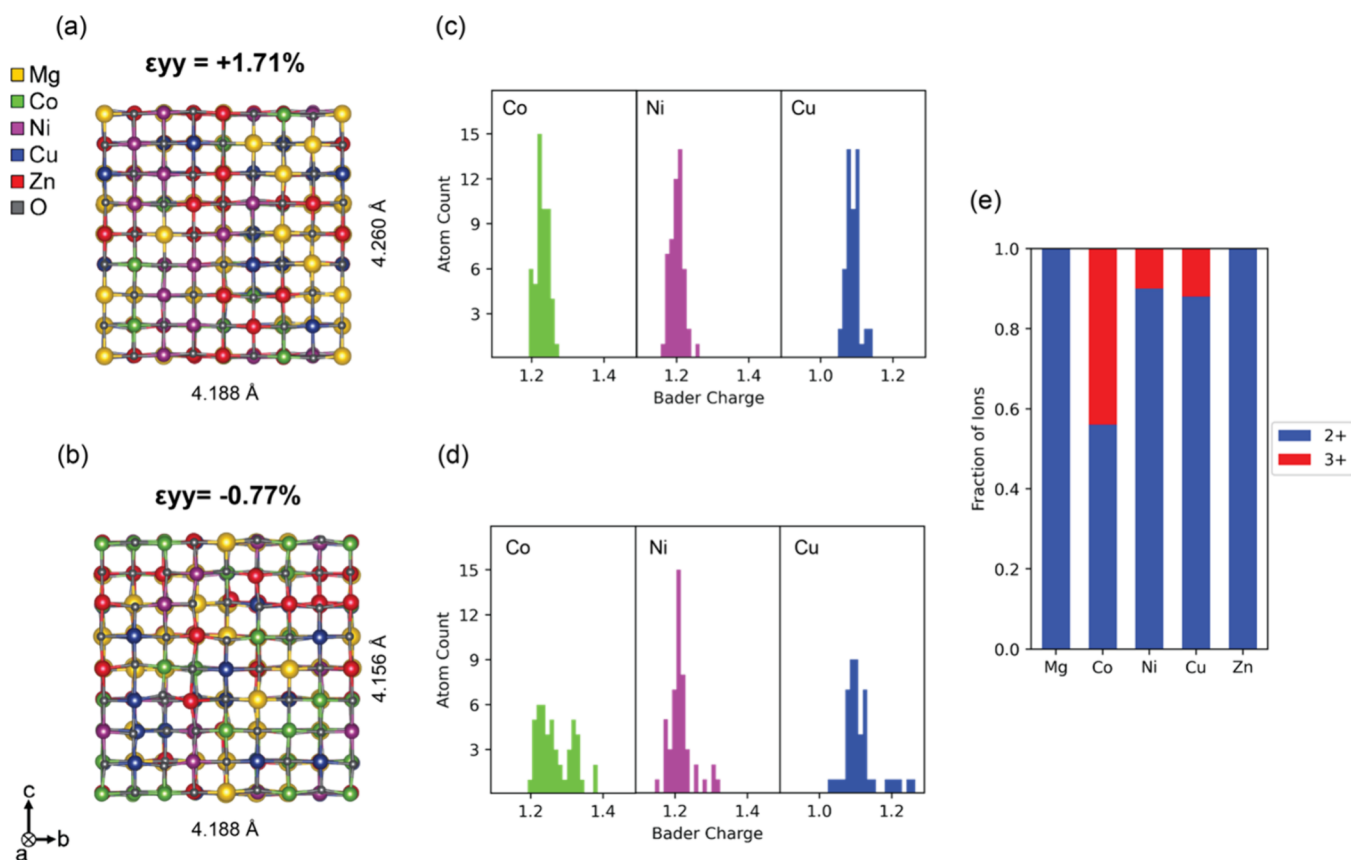
Figure 6. Results from DFT calculations of the pristine (J14 pris ) and defect (J14 vac ) SQSs corresponding to the high (500 °C) and low (200 °C) temperature films, respectively. Relaxed structures for J14 pris and J14 vac with corresponding lattice parameters and out-of-plane strain ( \epsilon_{yy} ) values are shown in parts a and (b), respectively. Bader charge distributions for J14 pris (c) and J14 vac (d) predict a significant change in the cobalt valence state when vacancies are present. The relative amounts of 2+ and 3+ cations within the J14 vac SQS are summarized in panel (e). Visualization was performed with VESTA. 46
