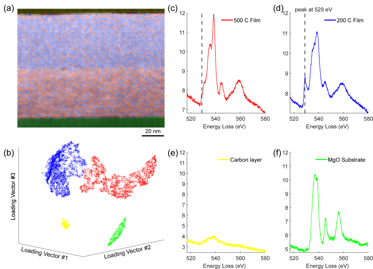
Figure 4. Unsupervised machine learning analysis of the STEM-EELS for the oxygen K edge. (a) Probe positions overlaid over the ADF-STEM image. The probe positions are categorized into four classes and colored based on the clustering results in (b) the visualization of the Gaussian mixture model (GMM) clustering results after the dimensionality reduction using non-negative matrix factorization and t-distributed stochastic neighbor embedding (t-SNE). (c–f) Class-averaged EELS spectra for four classes are primarily found in the 500 °C J14 film, 200 °C J14 film, carbon layer, and MgO substrate. The dashed line in panel (d) marks the position of the extra peak compared to panel (c).
