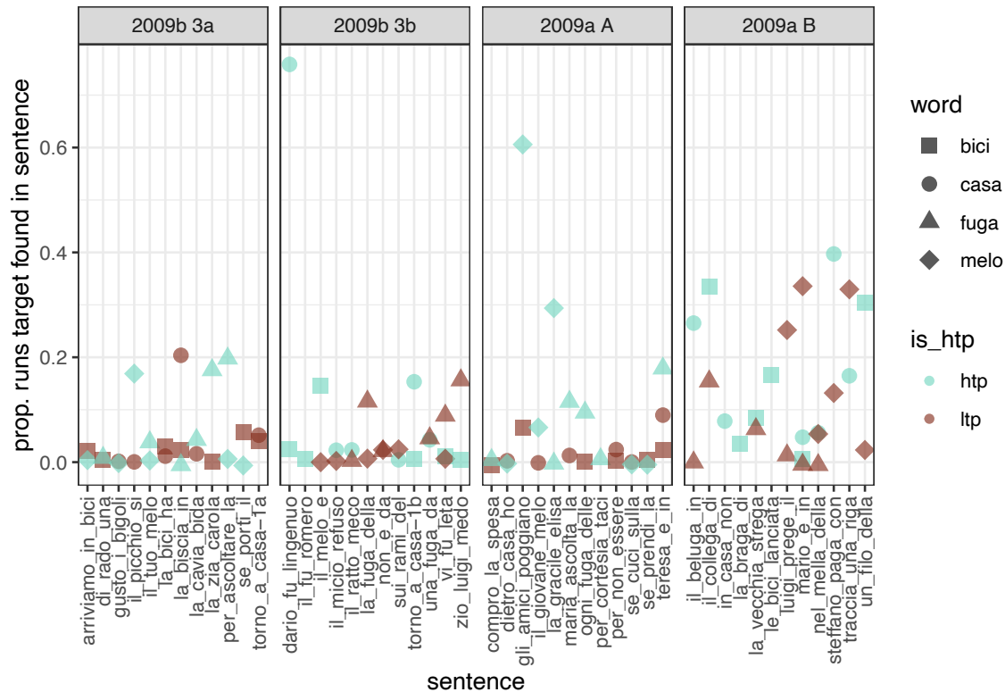
Figure 4. Exact discovery probability by sentence, each word, faceted by corpus. Sentences are indicated according to their first three words (see Supporting Online Materials for the full transcripts).
