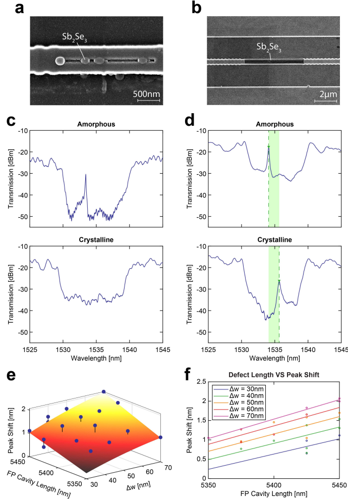
Fig. 5. Results of fabricated Fabry-Perot devices. (a)-(b) SEM Images of fabricated devices. Devices with \text{Sb}_2\text{Se}_3 (a) embedded and (b) evanescently coupled on the defect segment of a FP device. The poor quality of the filling of the \text{Sb}_2\text{Se}_3 in the embedded waveguide resulted in minimal effects after crystallization. The phase-shifted device shown in (b) is much less sensitive to alignment compared to the Bragg grating design (Fig. 4(a)). (c)-(d) Spectra of devices with \text{Sb}_2\text{Se}_3 deposited on top of the defect. The device in (c) shows an example of expected device behavior. Device in (d) exhibits the characteristic red shift of the passband. Passband peak shift was shown to be related to both FP cavity length and \Delta w of the Bragg reflectors and is shown in (e)-(f).
