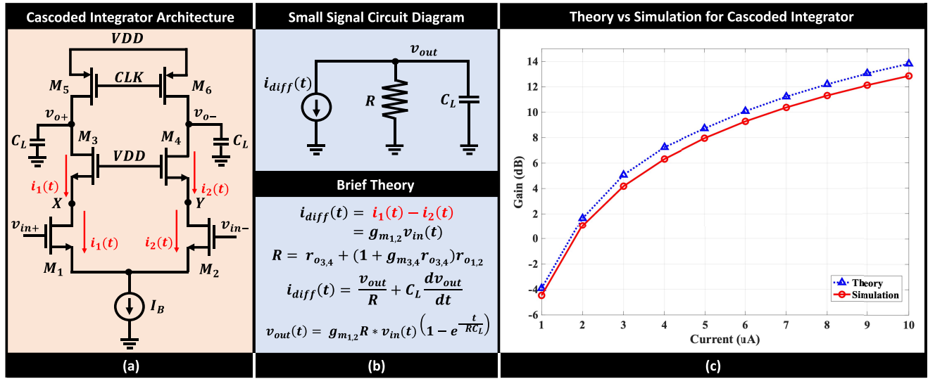
FIGURE 4. (a) Cascoded integrating amplifier architecture, (b) Small signal circuit diagram of the differential half circuit and crucial expressions, (c) Theory vs Simulation for cascoded integrator.
