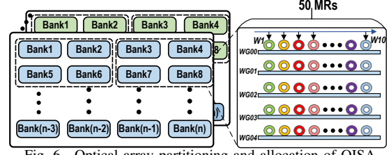
Fig. 6. Optical array partitioning and allocation of OISA.
