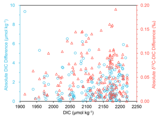
Figure 7. The absolute dissolved inorganic carbon (DIC) concentration differences (blue circles) and stable isotopic composition of DIC ( \delta^{13}\text{C} -DIC) differences (red triangles) against the DIC concentrations of discrete replicate samples collected during the cruise. 4 out of 186 pairs of duplicate measurements with a DIC concentration difference greater than 10 \mu\text{mol kg}^{-1} and \delta^{13}\text{C} -DIC difference greater than 0.2 \text{ ‰} were excluded in advance.
