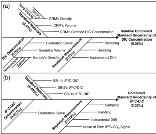
Figure 5. The sources of uncertainties for (a) the dissolved inorganic carbon (DIC) concentration and (b) the stable isotopic composition of DIC ( \delta^{13}\text{C} -DIC) measurements. Numbers in the brackets indicate the values of relative standard uncertainties for the DIC concentration and the standard uncertainties for the \delta^{13}\text{C} -DIC from different parts of sources.
