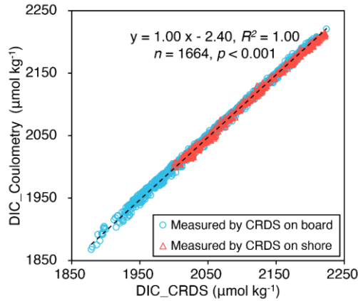
Figure 9. Dissolved inorganic carbon (DIC) concentration results measured by Cavity Ring-Down Spectroscopy (CRDS) on board (blue circle) or on shore (red triangle) plotted against DIC concentrations obtained through onboard coulometry measurements conducted by National Oceanic and Atmospheric Administration (NOAA)’s Atlantic Oceanographic & Meteorological Laboratory (AOML).
