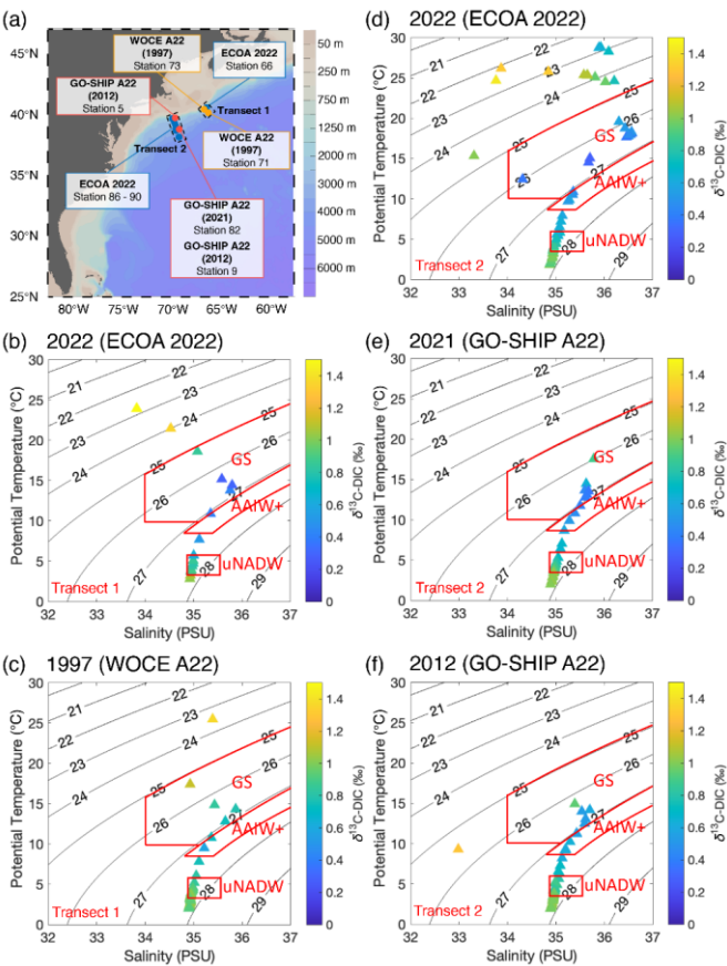
Figure 10. (a) Locations of selected deep-water stations with a water depth of > 2000 m for comparison with historical data. These stations were occupied during the East Coast Ocean Acidification (ECO) 2022 cruise (blue circles) and their nearby stations visited during the World Ocean Circulation Experiment (WOCE) A22 cruise in 1997 (yellow circles) and the Global Ocean Ship-based Hydrographic Investigations Program (GO-SHIP) A22 cruises in 2021
