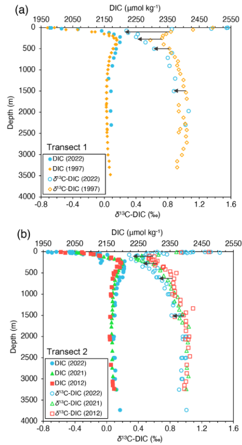
Figure 11. (a) The dissolved inorganic carbon (DIC) concentration and stable isotopic composition of DIC ( \delta^{13}\text{C-DIC} ) depth profiles measured during the East Coast Ocean Acidification (ECO) 2022 cruise (circles) at Transect 1 compared to that measured during the World Ocean Circulation Experiment (WOCE) A22 cruise in 1997 (diamonds) at the same location. (b) The DIC and \delta^{13}\text{C-DIC} depth profiles measured at Transect 2 during the ECOA 2022 cruise (circles) compared to that measured at the exact location in 2021 (triangles) and Station 9 in 2012 (squares) during the Global Ocean Ship-based Hydrographic Investigations
