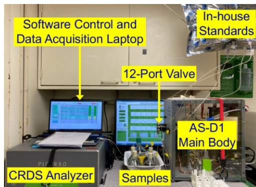
Figure 1. Photograph of the DIC/ \delta^{13}\text{C} -DIC analytical equipment installed onboard NOAA Ship Ronald H. Brown.
