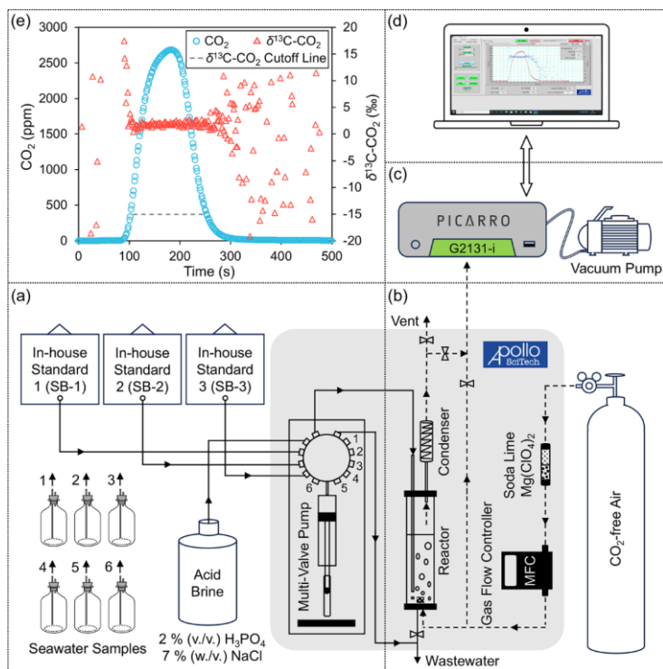
Figure 2. The schematic of the dissolved inorganic carbon (DIC) concentration and stable isotopic composition of DIC ( \delta^{13}\text{C-DIC} ) analytical system is subdivided into four distinct modules: (a) the sample injection module, (b) the \text{CO}_2 extraction module, (c) the detection module, and (d) the data processing and control module; and (e) a typical output showing data collected for one measurement of \text{CO}_2 concentration and stable isotopic composition of \text{CO}_2 ( \delta^{13}\text{C-CO}_2 ). Solid lines represent the flow of liquid, while dashed lines denote the flow of gas.
