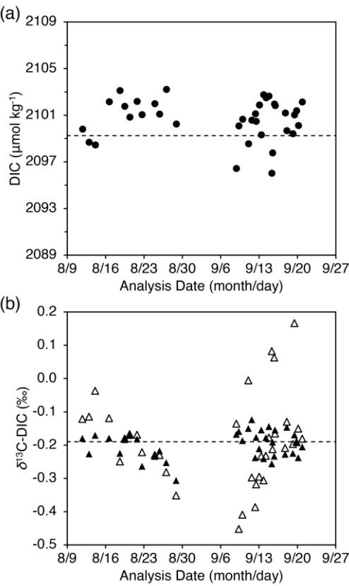
366 367 Figure 8. Measured (a) DIC concentrations (filled circles) and (b) stable isotopic composition of 368 DIC ( \delta^{13}\text{C-DIC} ) values (filled triangles) of certified reference materials (CRMs) from Batch 369 #188 relative to the analysis date ( n = 36 ). The dashed lines show the average DIC and \delta^{13}\text{C-DIC} 370 values of CRM #188 measured during the 40-day onboard period. The empty triangles indicate 371 raw \delta^{13}\text{C-DIC} values derived from single-point calibration without employing a time-dependent 372 linear regression method for correction, highlighting the long-term instrument drift.
