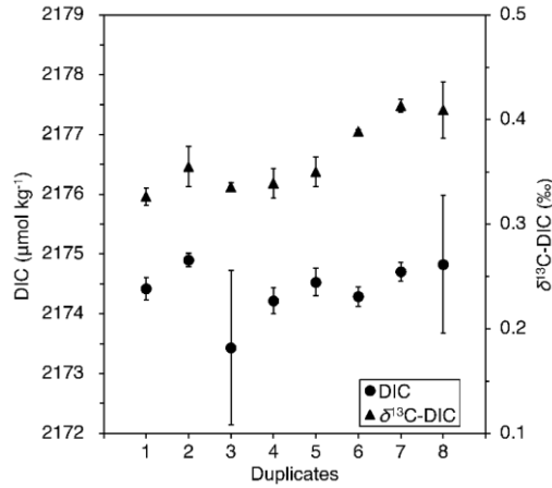
Figure 6. Dissolved inorganic carbon (DIC) concentrations and stable isotopic composition of DIC ( \delta^{13}\text{C-DIC} ) values of eight duplicate seawater samples collected at a depth of 226 m. The two ends of the error bar indicate the results of two rounds of measurements, and the symbol indicates the mean value.
