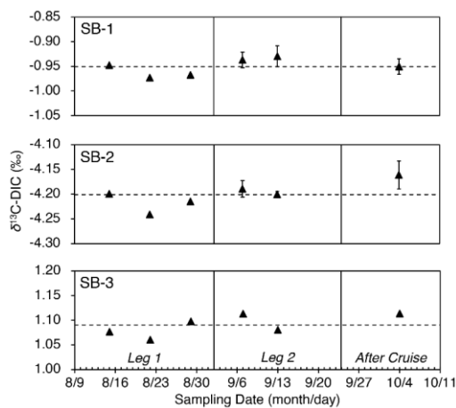
250 251 Figure 4. The stable isotopic composition of DIC ( \delta^{13}\text{C} -DIC) values measured by Isotope Ratio 252 Mass Spectrometry (IRMS) for three in-house standards periodically subsampled at sea and after 253 the cruise. The error bars indicate the standard deviation of \delta^{13}\text{C} -DIC for in-house standards 254 stored in different gas-tight bags. The dashed lines show the average \delta^{13}\text{C} -DIC value for each in- 255 house standard.
