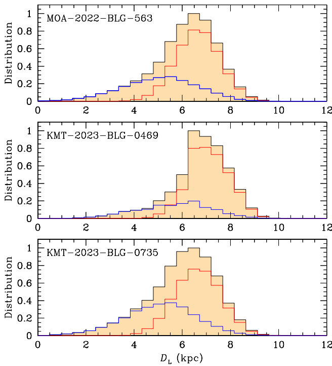
Fig. 10. Bayesian posteriors of the distances to the planetary systems. Notations are the same as those in Fig. 9.
