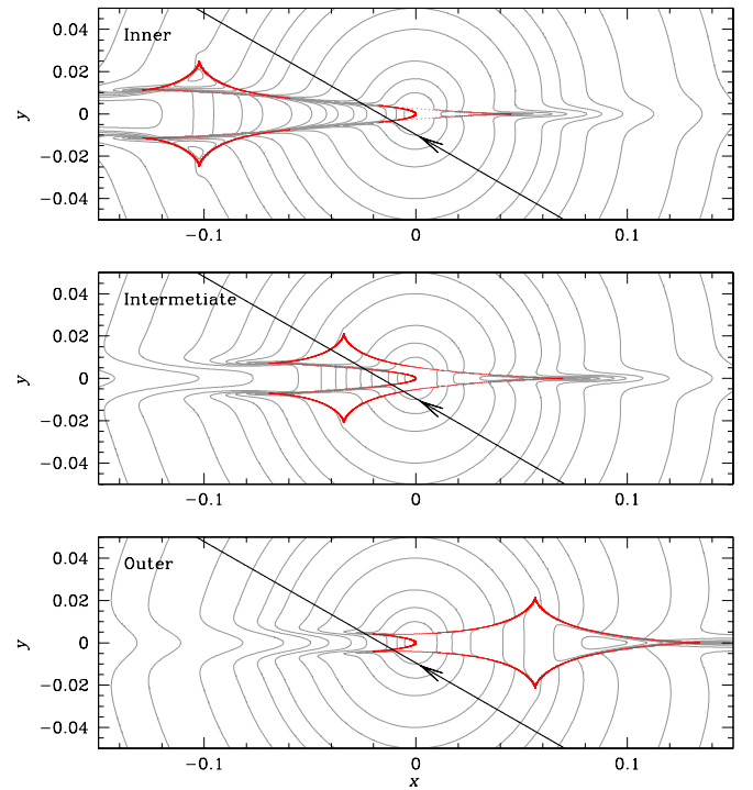
Fig. 5. Lens-system configurations of the inner (top panel), intermediate (middle panel), and outer (bottom panel) solutions for the lensing event KMT-2023-BLG-0469. Notations are same as those in Fig. 3.
