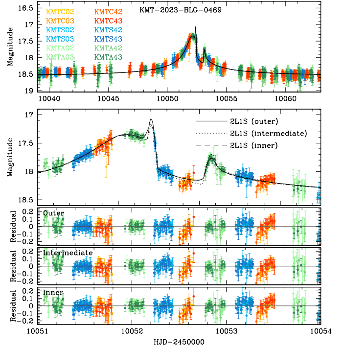
Fig. 4. Light curve of KMT-2023-BLG-0469. The solid, dotted, and dashed curves on the data points represent the models of the outer, intermediate, and inner 2L1S solutions, respectively.
