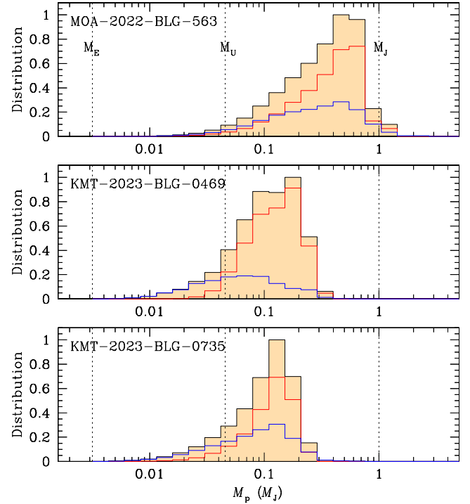
Fig. 9. Bayesian posteriors of the planet masses. The three dotted vertical lines represent the masses of Earth ( M_E ), Uranus ( M_U ), and Jupiter ( M_J ) of the Solar System. The curves drawn in red and blue indicate the contributions by the disk and bulge lens populations, respectively, and the black curve represents the sum of the contributions by the two lens populations.
