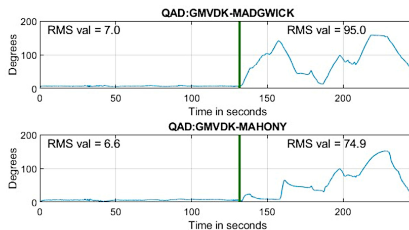
Figure 7. Quaternion angle difference (QAD) between GMVDK and Madgwick’s algorithm (top panel), and quaternion angle difference (QAD) between GMVDK and Mahoney’s algorithm (bottom panel). In each case, the RMS value of QAD for the intervals before and after the vertical dividing line is indicated.
