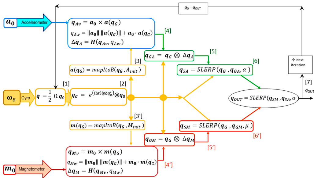
Figure 1. Flow of information within a single iteration of the GMVD orientation estimation algorithm. The numbers in square brackets indicate the computation steps.
