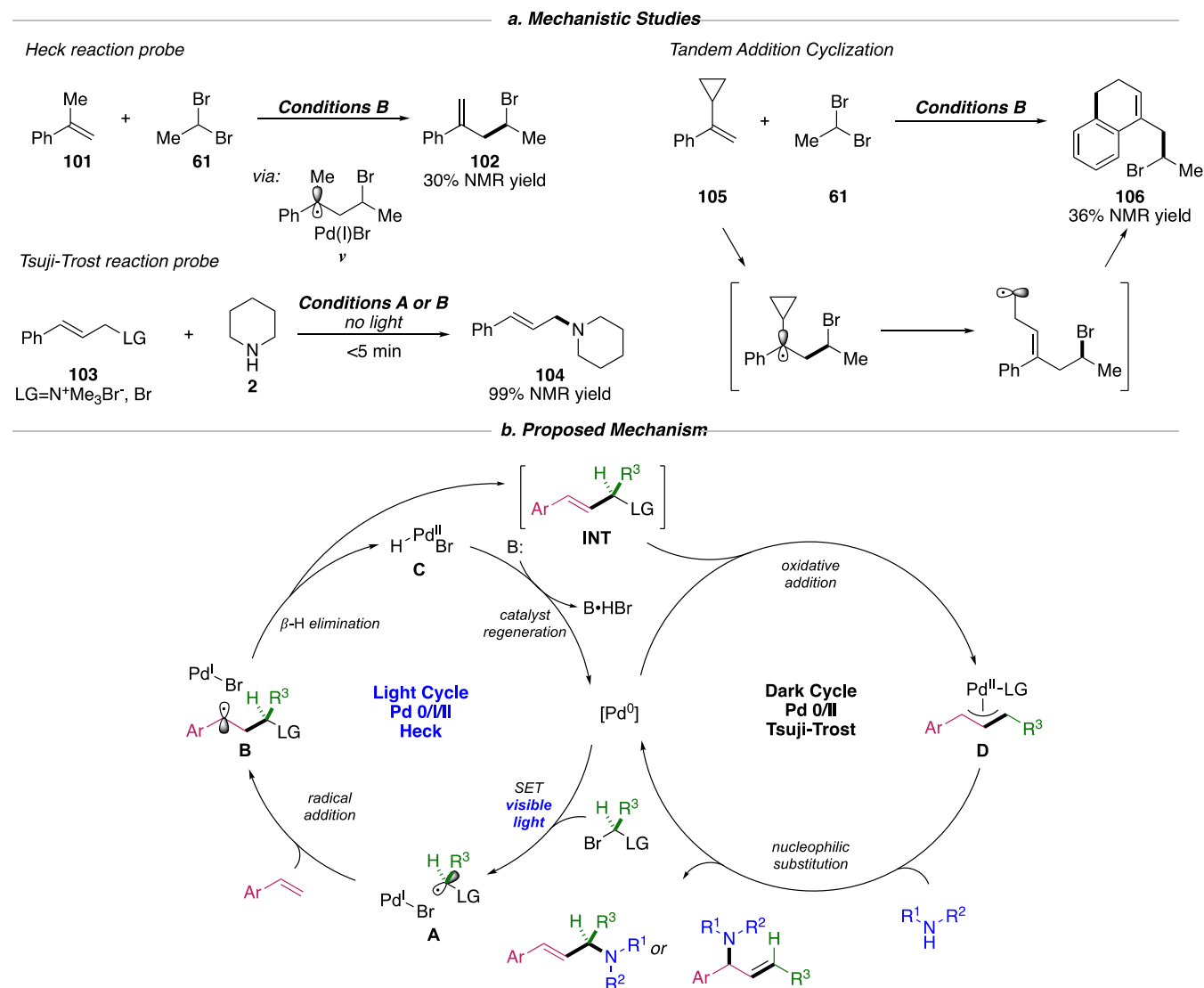
Scheme 7. Elucidation of Mechanism
