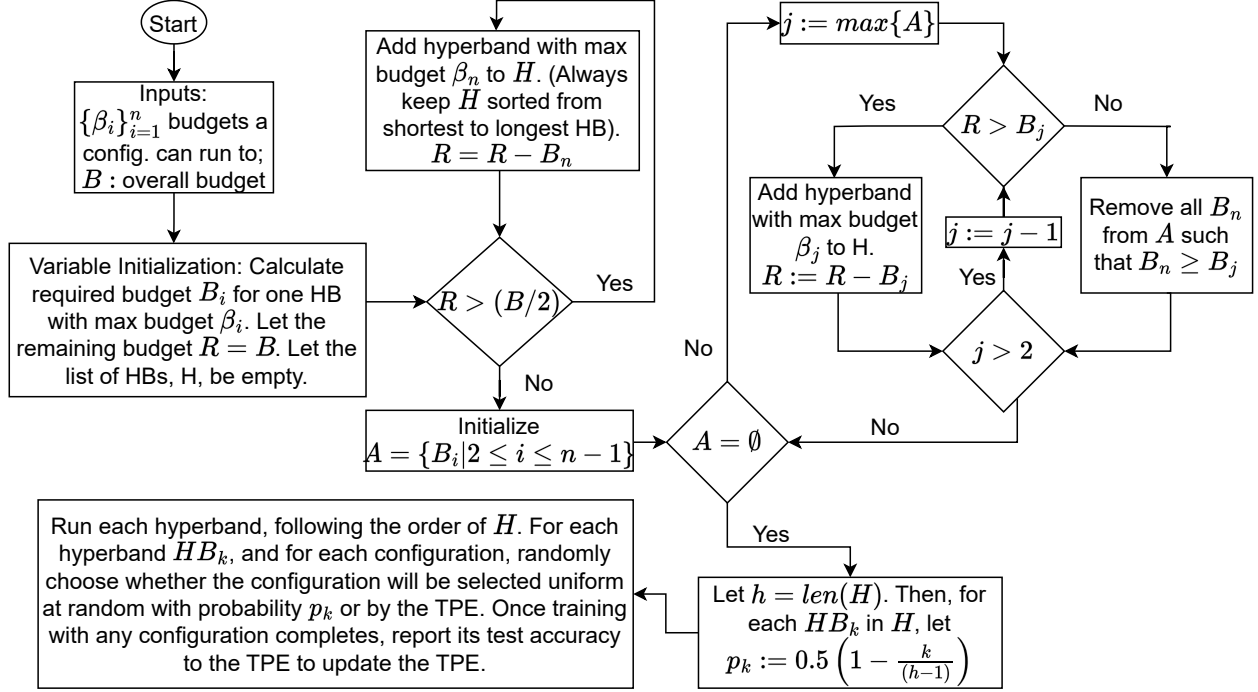
Figure 1: POCA flowchart.
