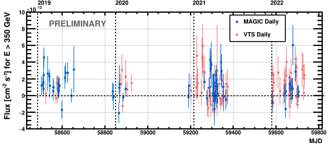
Figure 1: Daily light curves from 2019 to 2022 from MAGIC (blue points) and VERITAS (red points).
