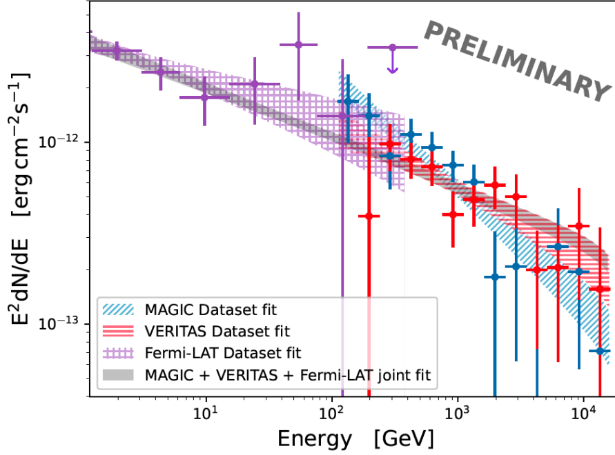
Figure 3: Spectral energy distribution between 2019 and 2022 combining data from MAGIC (blue points), VERITAS (red points) and Fermi-LAT (purple points). The fit to the MAGIC (blue band), VERITAS (red band), and Fermi-LAT (purple band) can be described by a power law. The joint fit (gray band) can be also described by a power-law.
