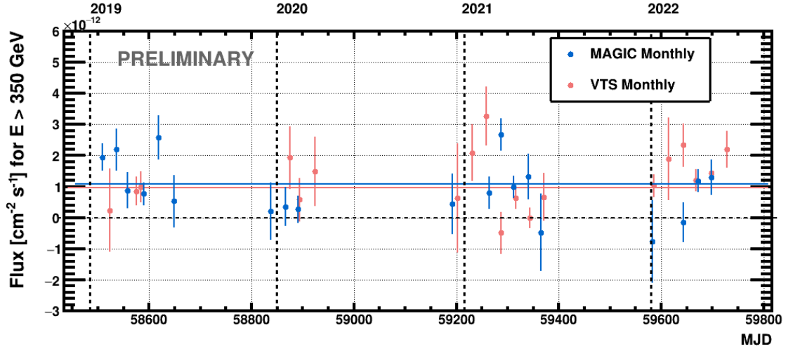
Figure 2: Monthly light curves from 2019 to 2022 from MAGIC (blue points) and VERITAS (red points). The mean integral flux is obtained by a fit to a constant to the monthly light curves for MAGIC (blue line) and VERITAS (red line).
